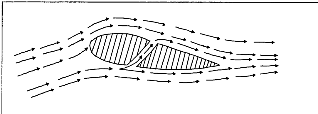
FIGURE 2.48 FIXED SLOT
