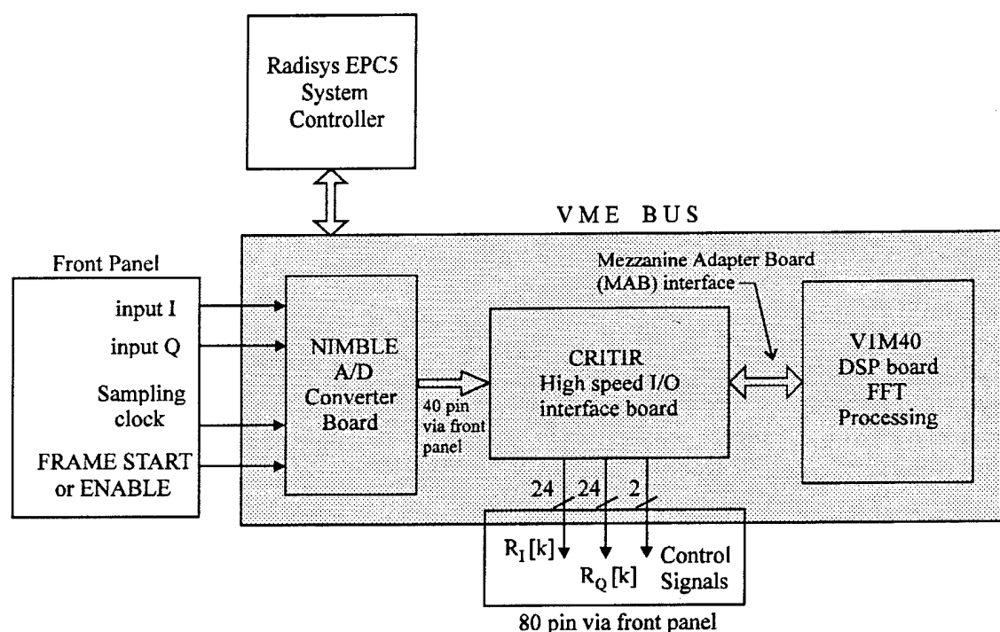
Fig.3.1. Overall system block diagram of FFT-based demodulator
