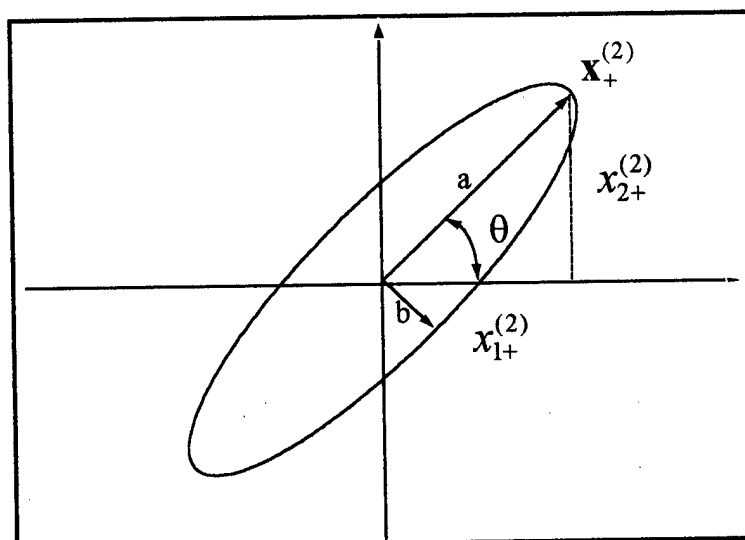
Figure 3.3 ELLIPSE ORIENTATION
