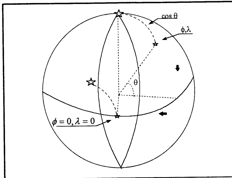
Figure 4.2 NORTH POLE ROTATION
