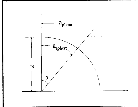
Figure 3.1 PROJECTION GEOMETRY
