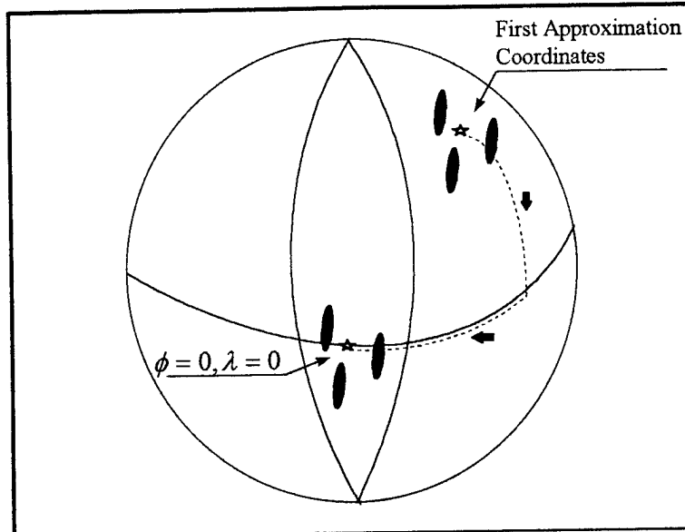
Figure 4.1 COORDINATE TRANSFORMATION
