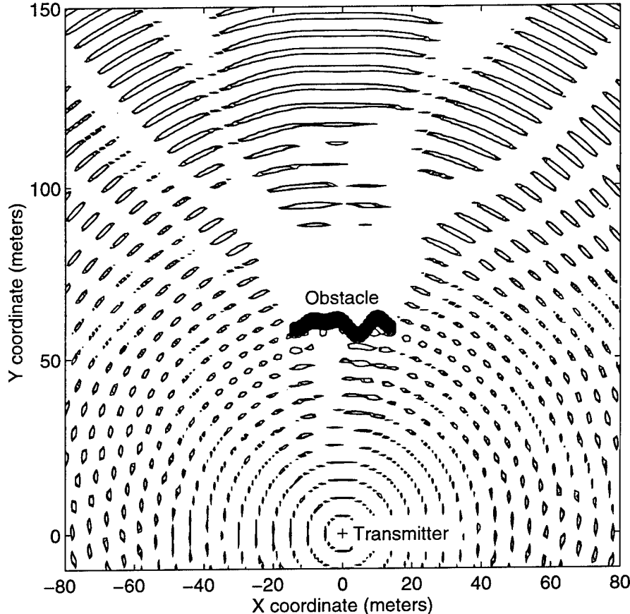
Figure 3: Overview of a signal impinging on a large obstacle
