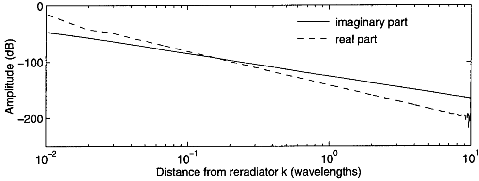
Figure 34: Values of the coupling elements \gamma_{kl} as a function of the distance between reradiators r_{kl} .
