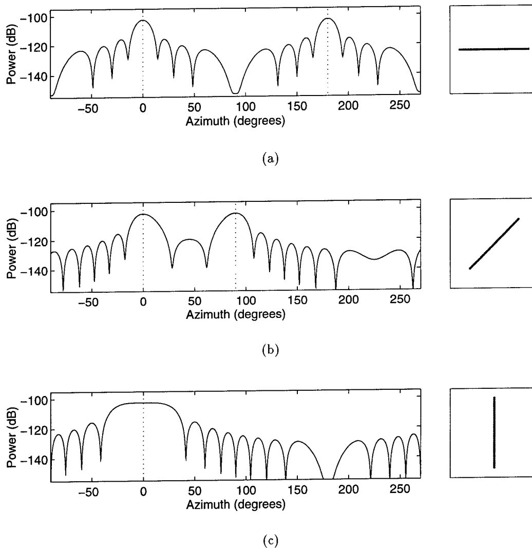
Figure 16: Reflection beam generated by a line source with orientations relative to the transmitter signal of (a) 0° (broadside), (b) 45°, and (c) 90° (in line or endfire). Dotted lines show positions of both the main lobe (at 0° azimuth) and reflection lobe (if present). Line source orientations are also plotted in small boxes on righthand side.
