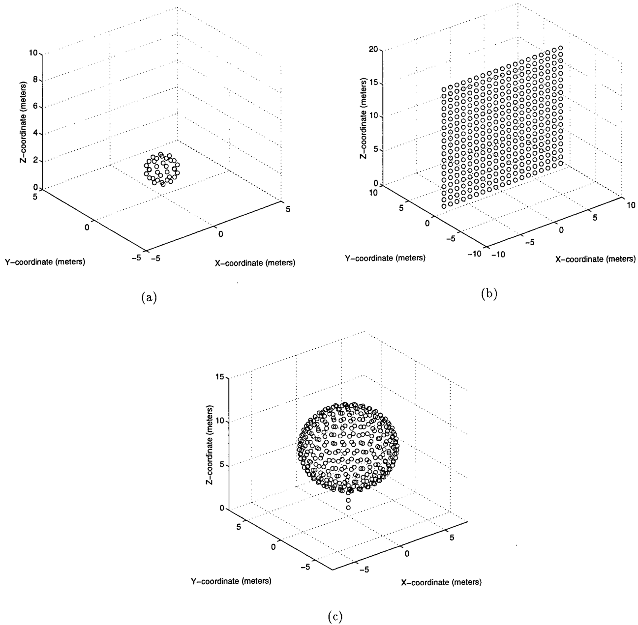
Figure 37: Shape of multipath sources showing reradiator positions for (a) small scatterer model, (b) tree model, and (c) large reflector model.
