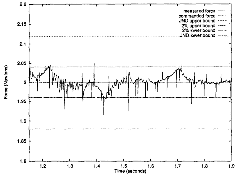
Figure 17. Steady-State Response with a 2 N Reference Force
