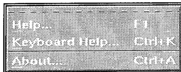
Figure 16. Help Menu
