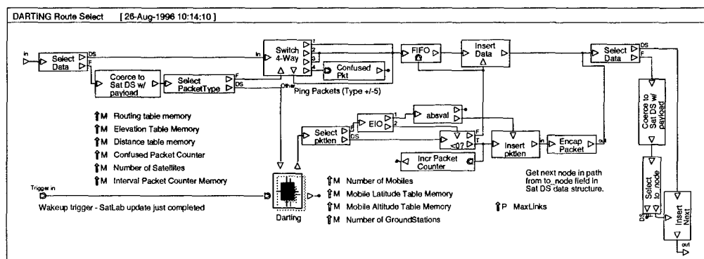
Figure 37: Darting Router
