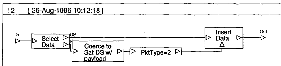
Figure 36: Bellman-Ford PacketType Kludge
