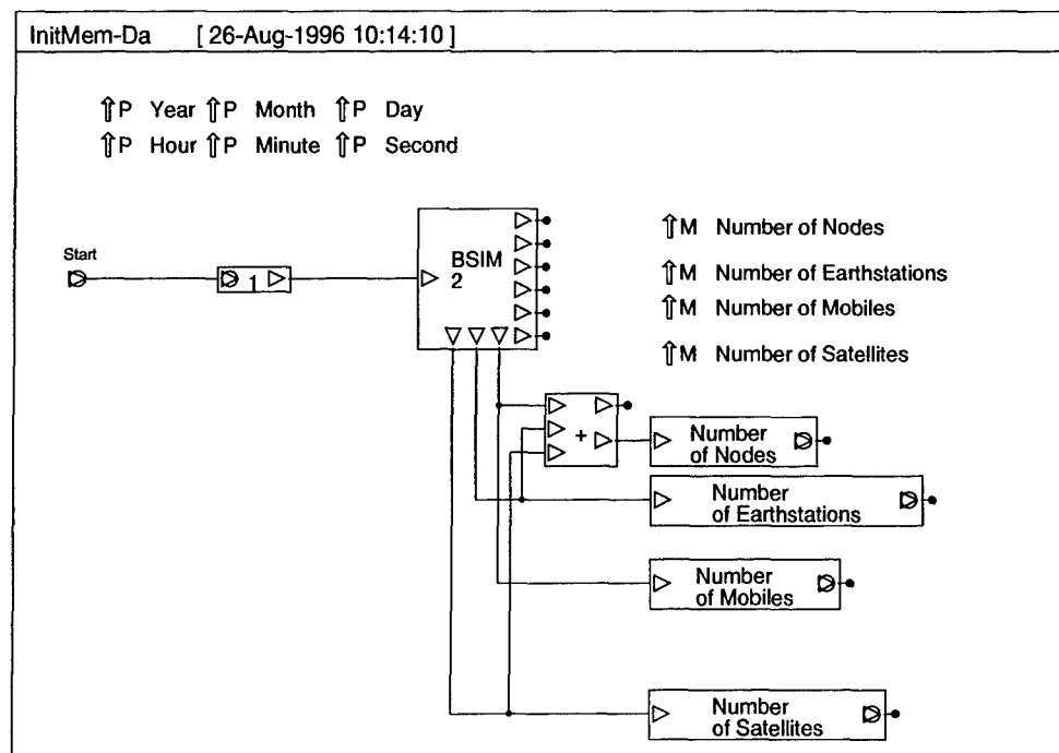
Figure 28: SatLab Memory Initialization
