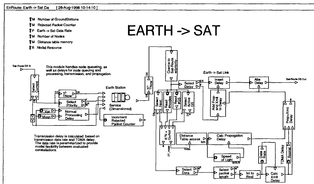
Figure 35: Uplink Delay (Earth-Sat) Block
