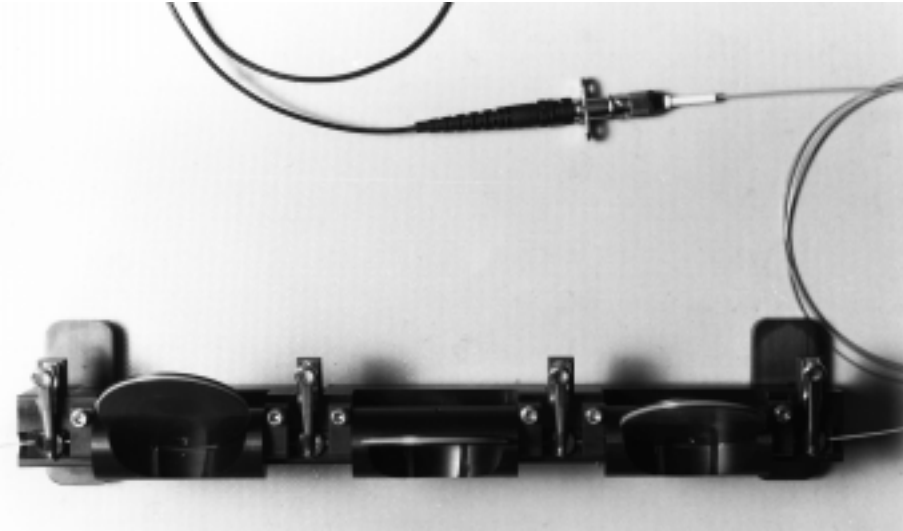
Figure 15. Top view of the MPC1000 polarization controller with three turns per disc.
