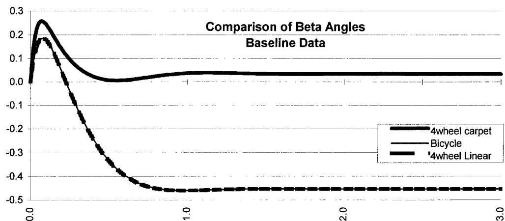
Figure 4.12 Sideslip angle response to 1^\circ step steer input at 60 kph
