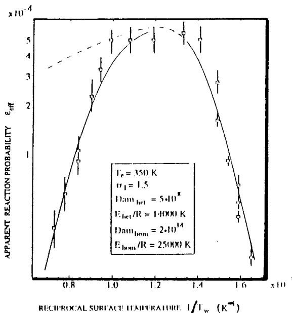
Fig. 8 \text{TiO}_2(\text{s}) deposition rate data (reported as an apparent first order heterogeneous rate constant) from \text{TTIP}/\text{O}_2/\text{N}_2 mainstream showing 'best-fit' deposition rates (after Rosner, Collins and Castillo, 1993, Castillo and Rosner, 1994) predicted using chemical sublayer (CSL-) theory, allowing for homogeneous consumption of TTIP within thermal BL.
