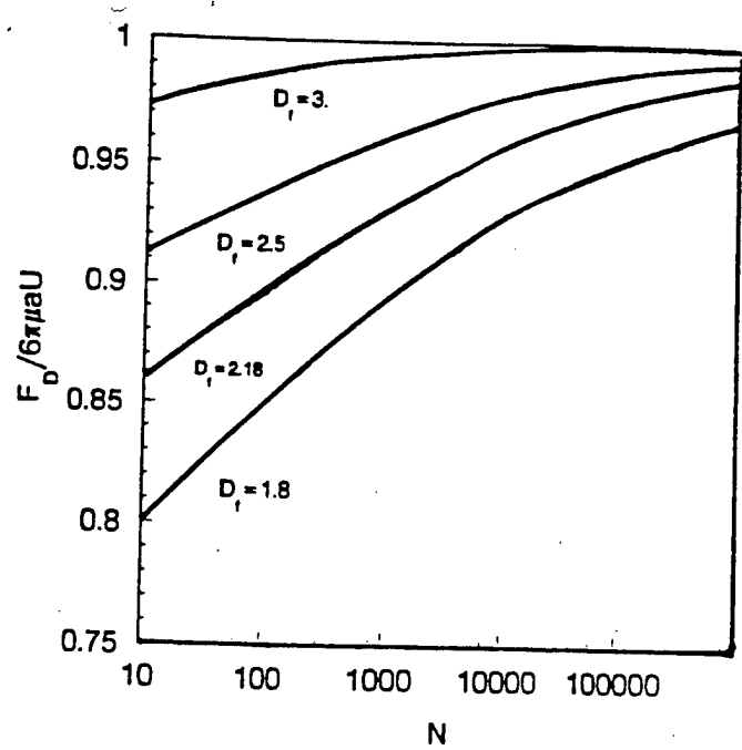
Fig. 2 Drag reduction associated with effective permeability for a quasi-spherical "fractal" aggregate comprised of N primary spheres in the continuum regime ( a = R_{max} = \{(3/2) \cdot [D_f + 2] / D_f\}^{1/2} R_{gyration} ) (after Tandon and Rosner, 1994)
