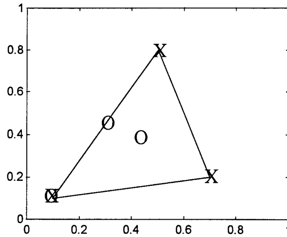
Figure 12: Three Material Mixtures in Two Spectral Bands
