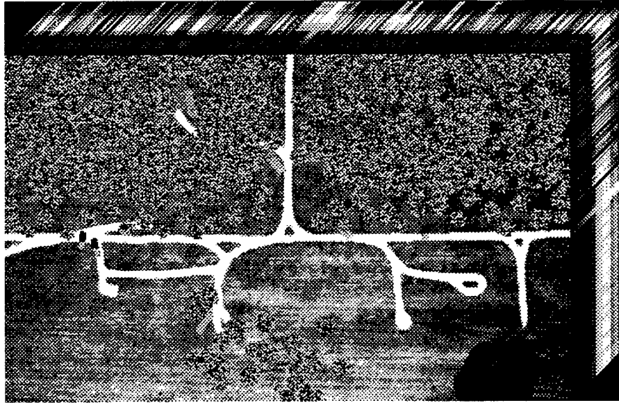
Figure 2: Image Cube
