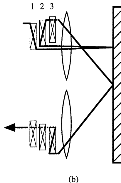
Fig. 4. (a) is a schematic side view of an optically interconnected MIN for a square array of N=16 nodes: The integrated plane of electronic switching and OE I/O are schematically depicted as 2 \times 2 crossbars. An example path from the upper input port of switch I-1 to the upper output port of switch II-3 is shown. (b) is a schematic side view of the interleaved retro-reflective partitioning of (a). The stages of nodes, represented here as 2 \times 2 crossbars, are interleaved. The same example path is depicted as in (a). The switching functions are expanded for illustrative purposes. In practice, all switches would be integrated into the single opto-electronic backplane. For large networks, this concept extends to one lens for each chip in the opto-electronic backplane, where each OEIC contains k \times k nodes. Furthermore, each node contain one switch for each stage present in the Sliding Banyan.
