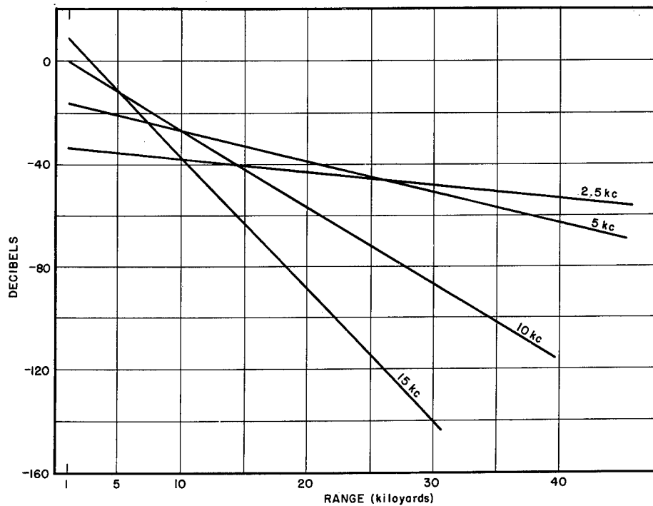
Fig. 1 - Equipment merit as a function of range (relative to 10 kc at 1 kiloyard)
