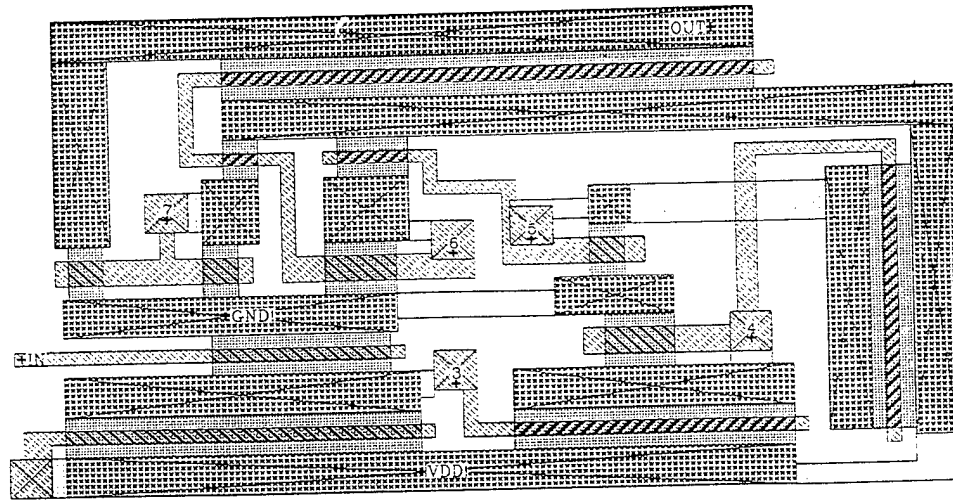
Figure 5-4 Receiver Layout
