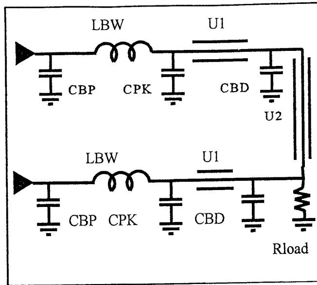
Figure 2-10 Schematic Diagram of Interconnect Circuit
