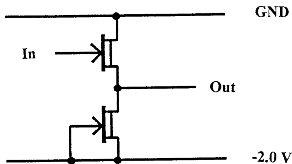
Figure 4-1 Source-Follower Buffer Design
