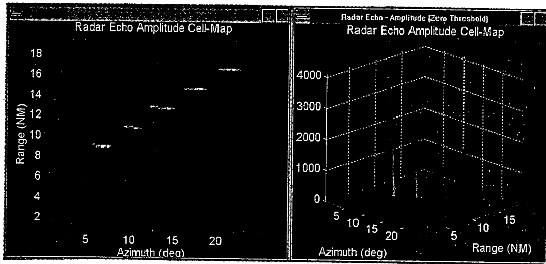
Figure A.25 Amplitude Cell-map with Zero Threshold
