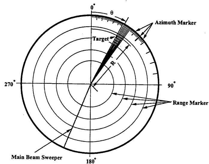
Figure 3.12 Key Elements on a Simulated PPI Display
