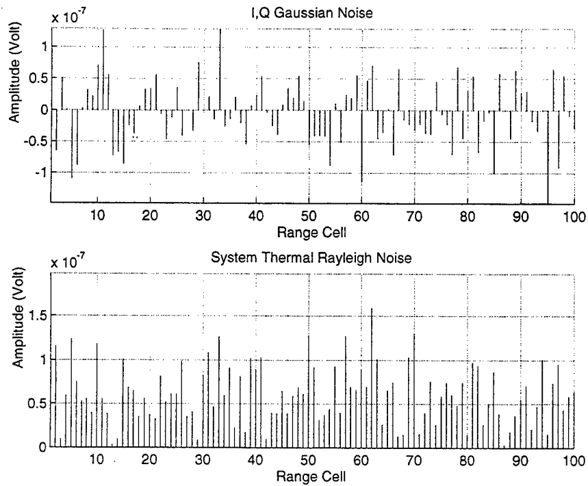
Figure 3.7 Gaussian and Rayleigh Noises
