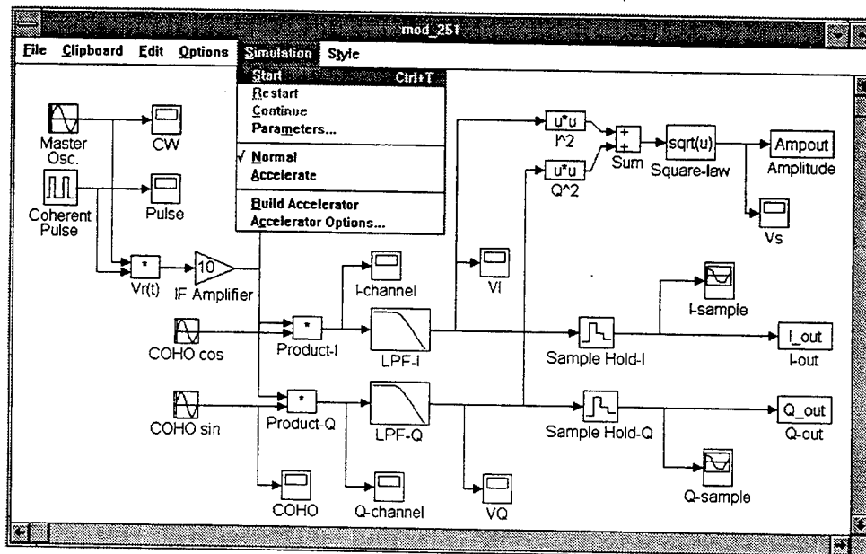
Figure A.10 The SIMULINK Synchronous Detector Model
