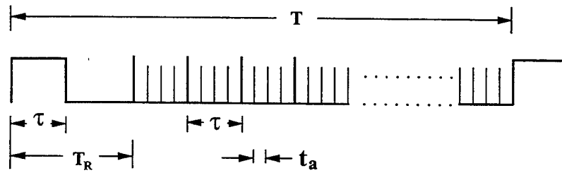
Figure 2.2 Definition of Radar Waveform
