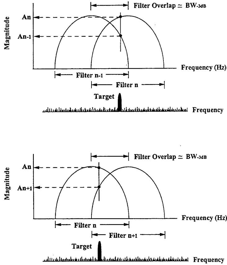
Figure 2.11 Target Response Doppler Frequency
