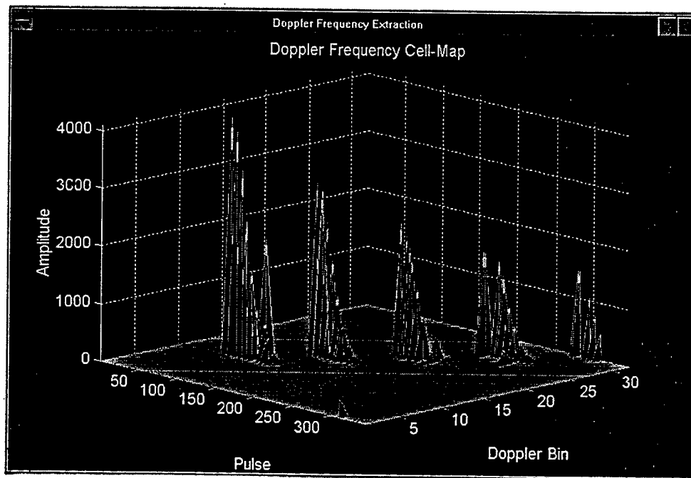
Figure 3.16 Amplitude as a Function of Range-Doppler-Azimuth
