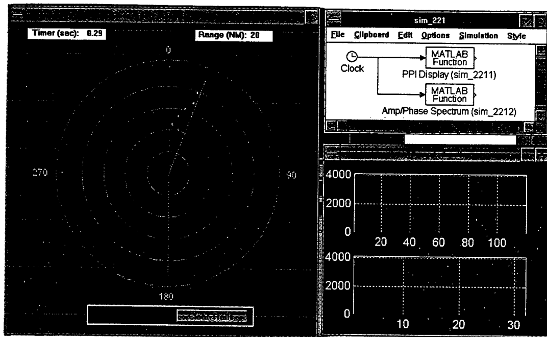
Figure 3.14 Simulated PPI Display for Radar Processing
