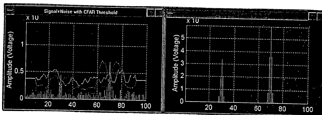
Figure A.12 CFAR and Threshold Detection Model
