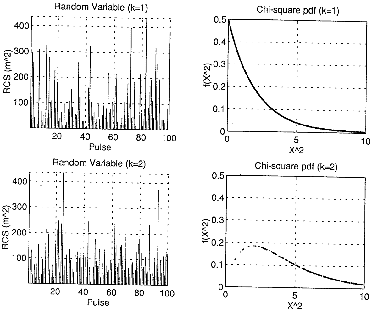
Figure 3.2 Random Variable and pdf of RCS Fluctuation
