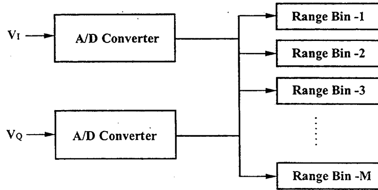
Figure 2.8 Block Diagram of A/D Converter
