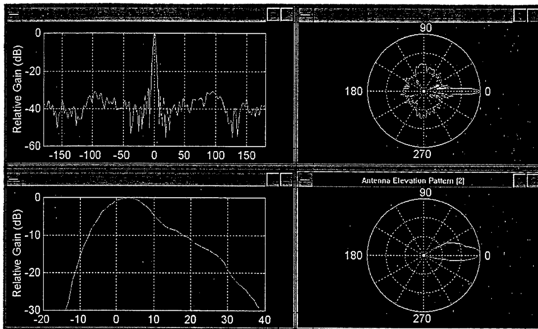
Figure A.8 Digitized Antenna Radiation Patterns
