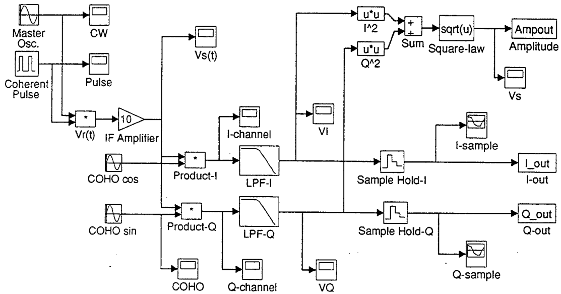
Figure 2.7 Synchronous Detector Model
