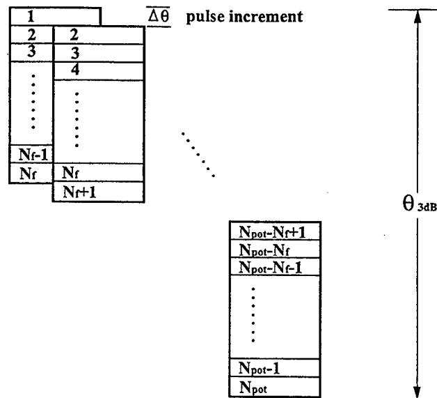
Figure 2.14 Moving Window Postdetection Integration
