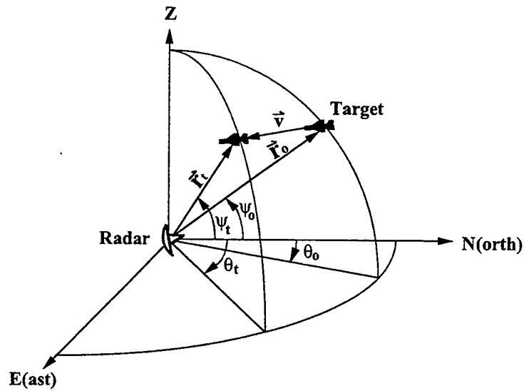
Figure 3.1 Target Trajectory
