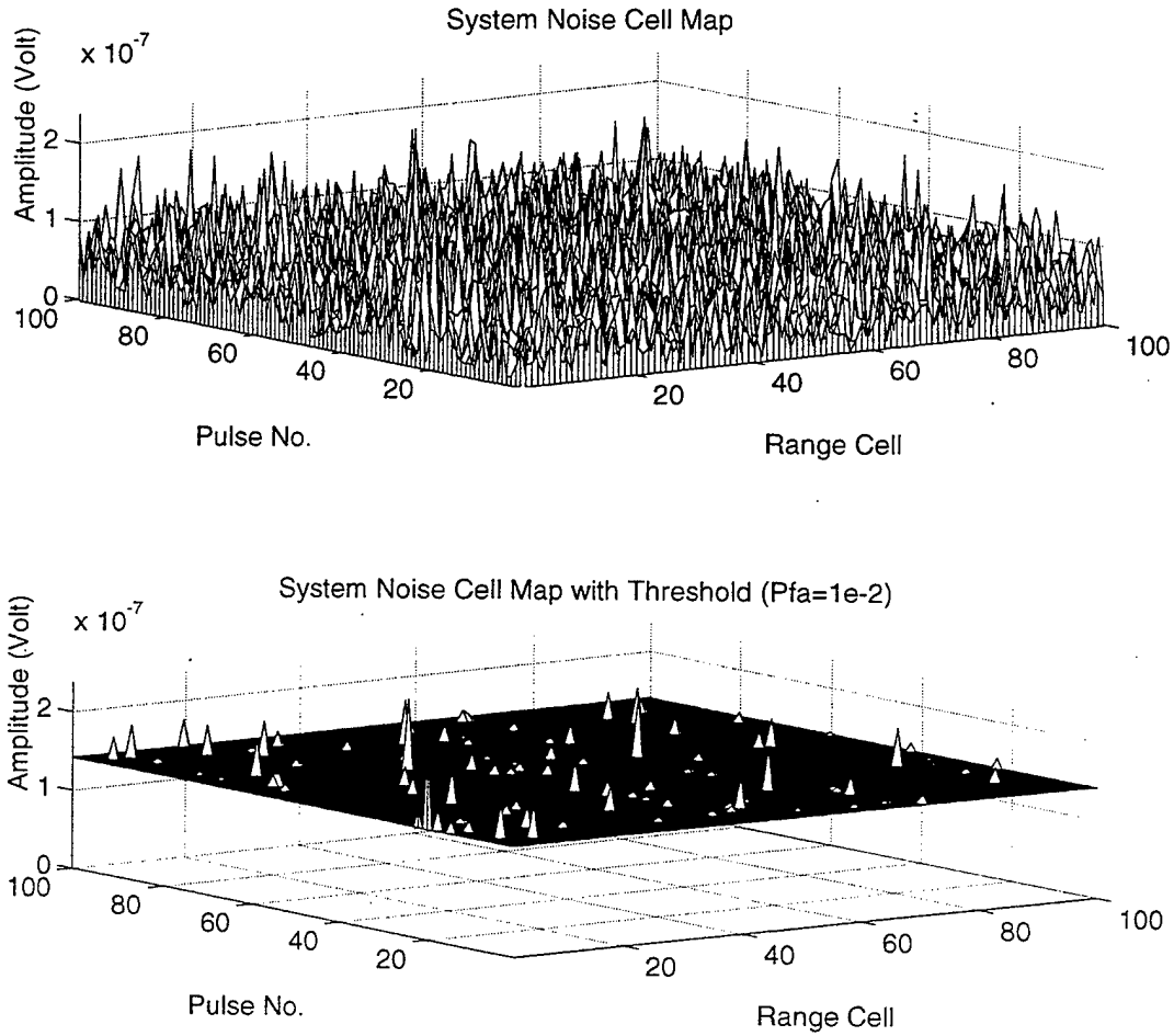
Figure 3.9 Simulated System Thermal Noise
