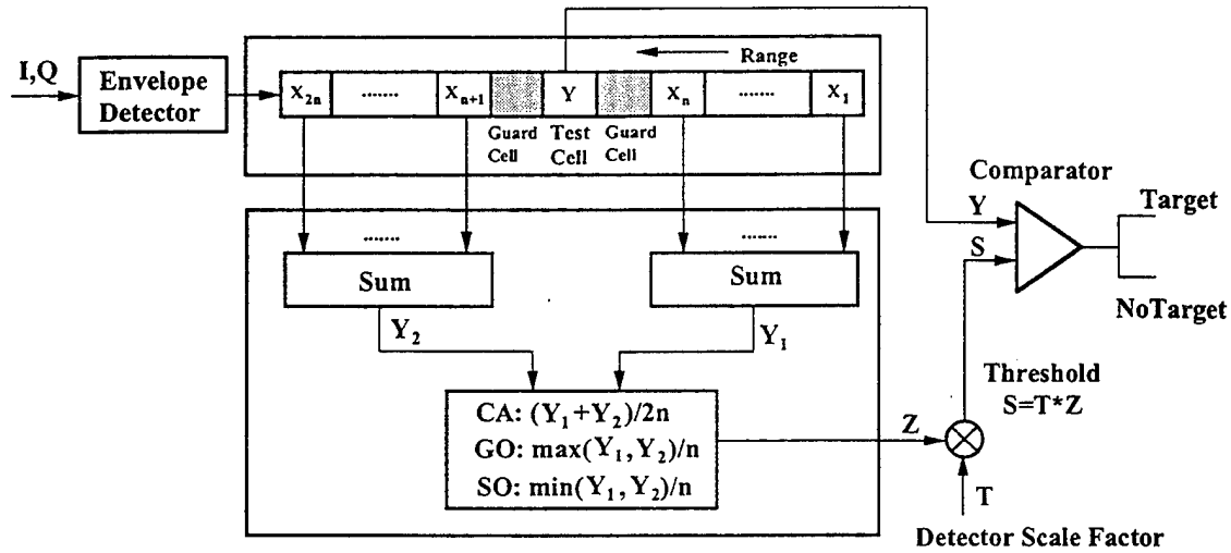
Figure 2.13 Block Diagram of the Mean-level CFAR Processor
