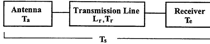
Figure 2.5 Temperature Components in a Cascade Receiving System
