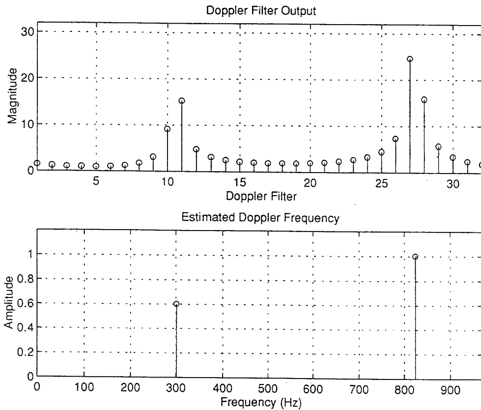
Figure 2.12 Simulated Target Response Doppler Frequency
