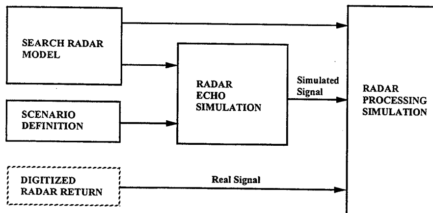
Figure 1.1 Software Structure
