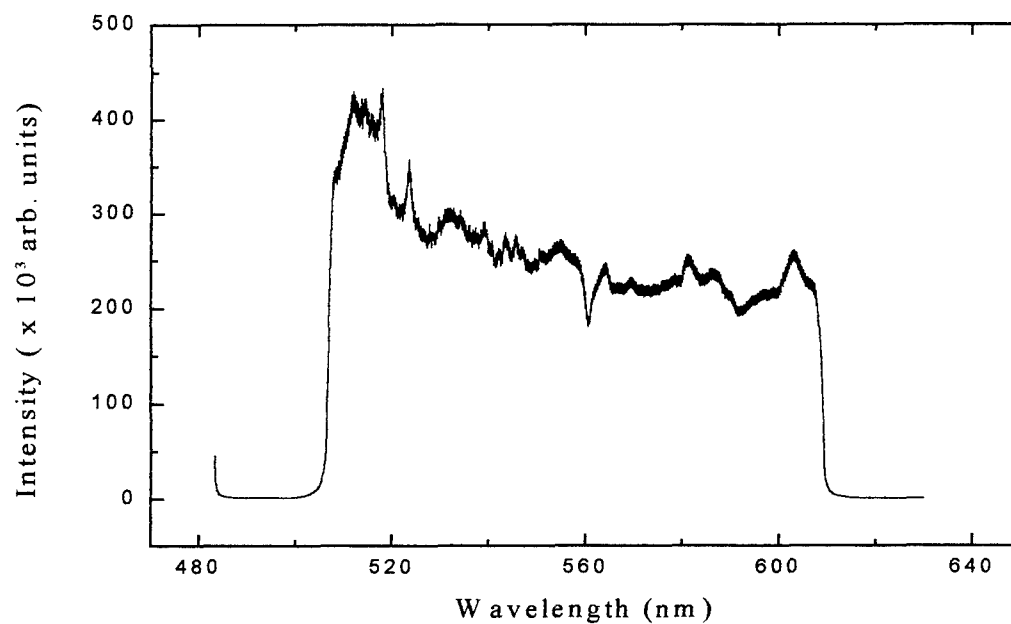
Figure D.21 \text{CCl}_4 Spectrum Covering 505 - 605 nm (100 \mu\text{m} slit width)
