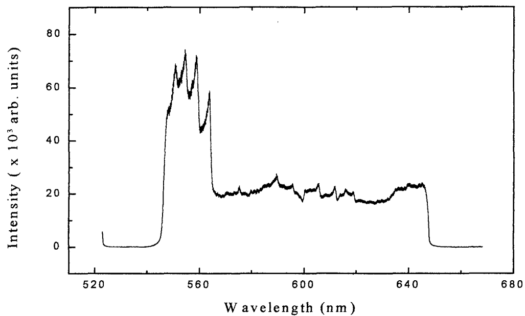
Figure D.19 \text{C}_2\text{Cl}_4 Spectrum Covering 545 - 645 nm
