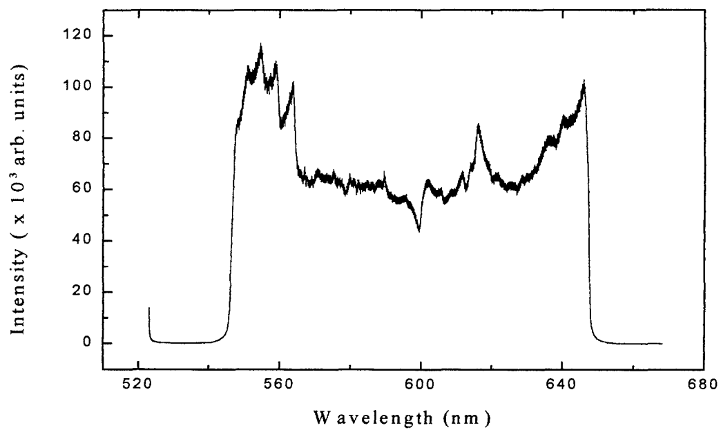
Figure D.20 \text{C}_2\text{HCl}_3 Spectrum Covering 545 - 645 nm
