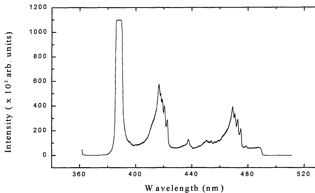
Figure D.35 \text{C}_2\text{Cl}_4 Spectrum Covering 385 - 485 nm
