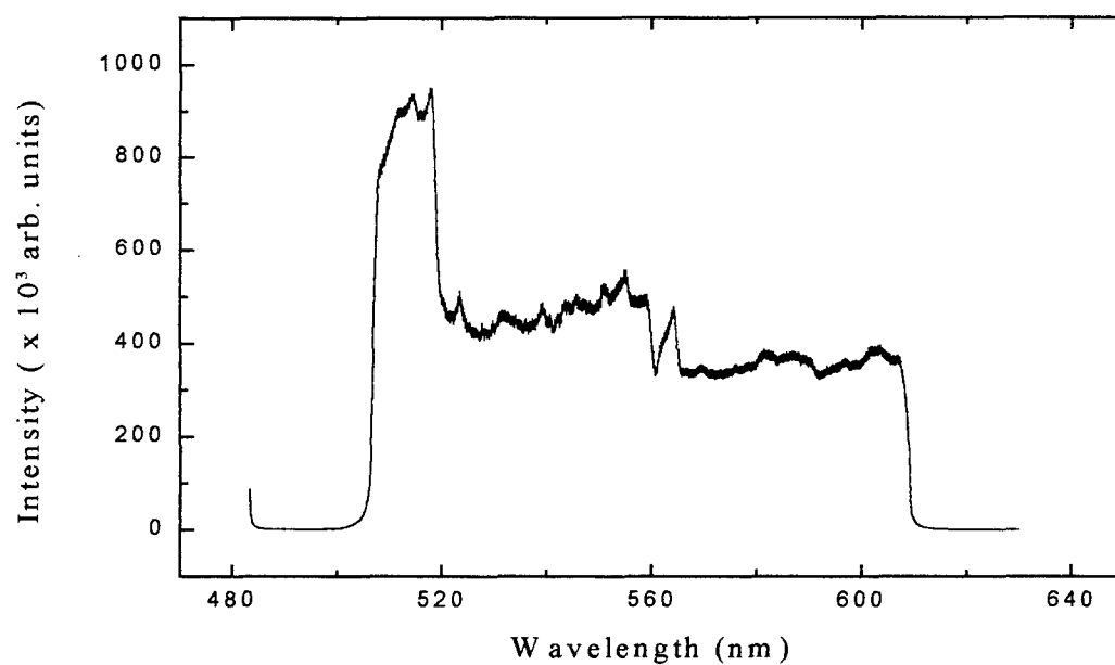
Figure D.22 \text{CHCl}_3 Spectrum Covering 505 - 605 nm (100 \mu\text{m} slit width)
