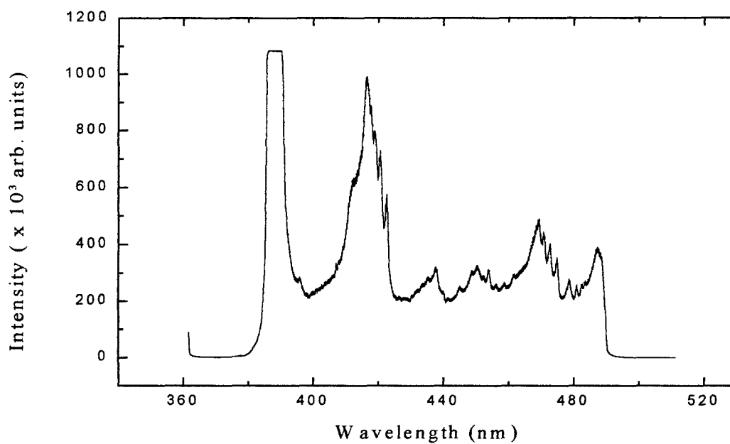
Figure D.36 \text{C}_2\text{HCl}_3 Spectrum Covering 385 - 485 nm
