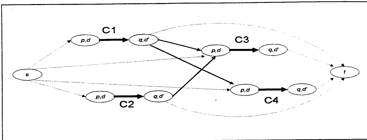
Figure 4. Network representation of the maximum flow model.
