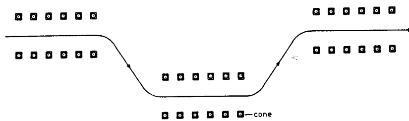
Fig. 3. Schematic representation of the vehicle clearing course.
