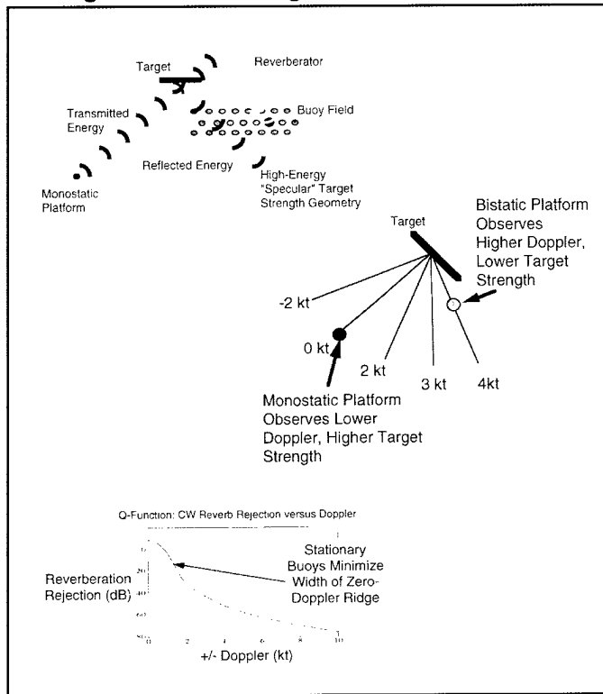
Figure 39 Processing for Distributed Fields
