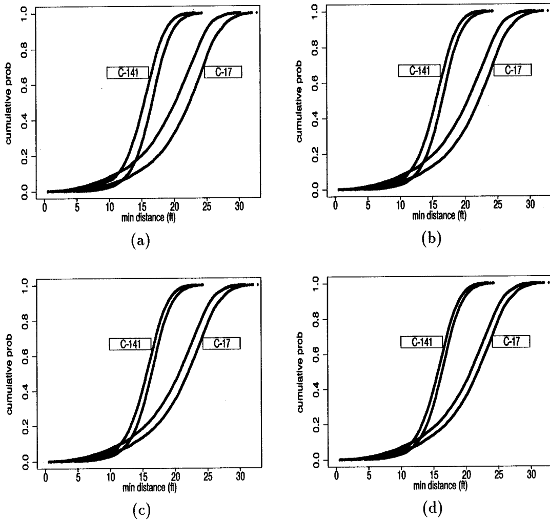
Figure D.3 Comparing Bootstrap Confidence bounds between C-141 vs. March heavy C-17: (a) 90% bootstrap confidence bounds (b) 80% bootstrap confidence bounds, (c) 70% bootstrap confidence bounds, (d) 60% bootstrap confidence bounds.
