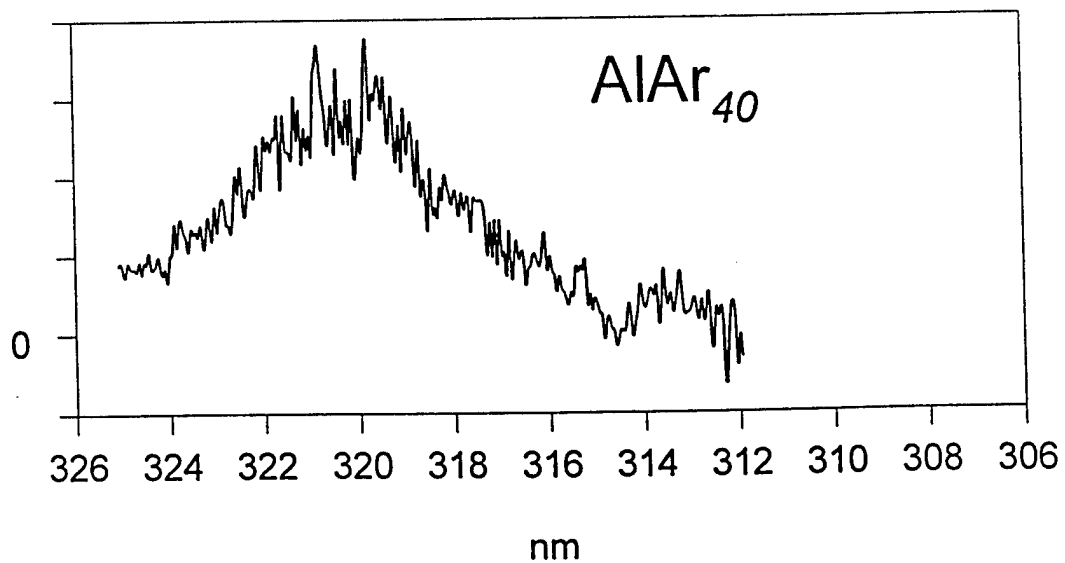
Figure 4c. R2PI spectra of AlAr n , n = 25, 34, and 40.
