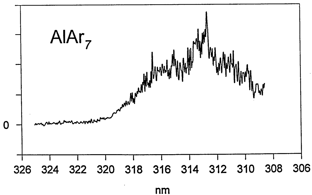
Figure 4a. R2PI spectra of AlAr n , n=4,7.
