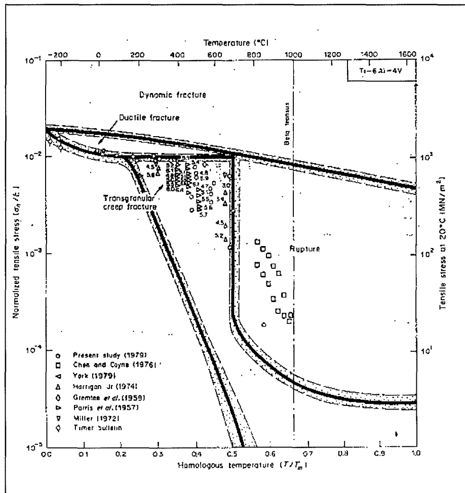
Figure 3.1 Fracture Mechanism Map for \alpha+\beta Alloy Ti-6Al-4V [18]
