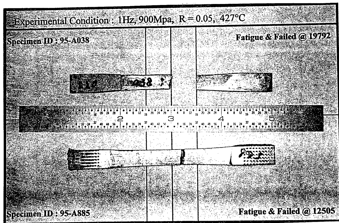
Figure A.4 Specimen Nos. 95-038 and 95-885 (1Hz Test)
