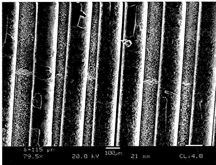
Figure 4.17 Matrix Cracking without Damage of the Fibers
