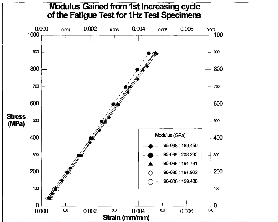
Figure 4.3 Modulus measured at the first fatigue cycle under 1Hz.
