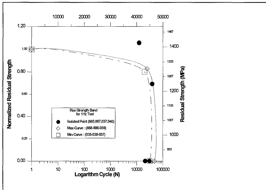
Figure 4.31 Normalized Residual Strength vs. Logarithm Cycles
