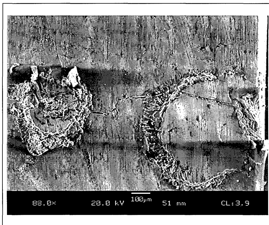
Figure 4.47 Welding Site Before R.S. Test
