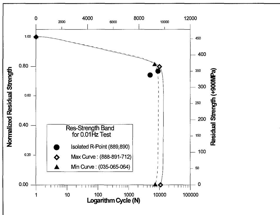
Figure 4.36 Normalized Residual Strength vs. Logarithm Cycles
