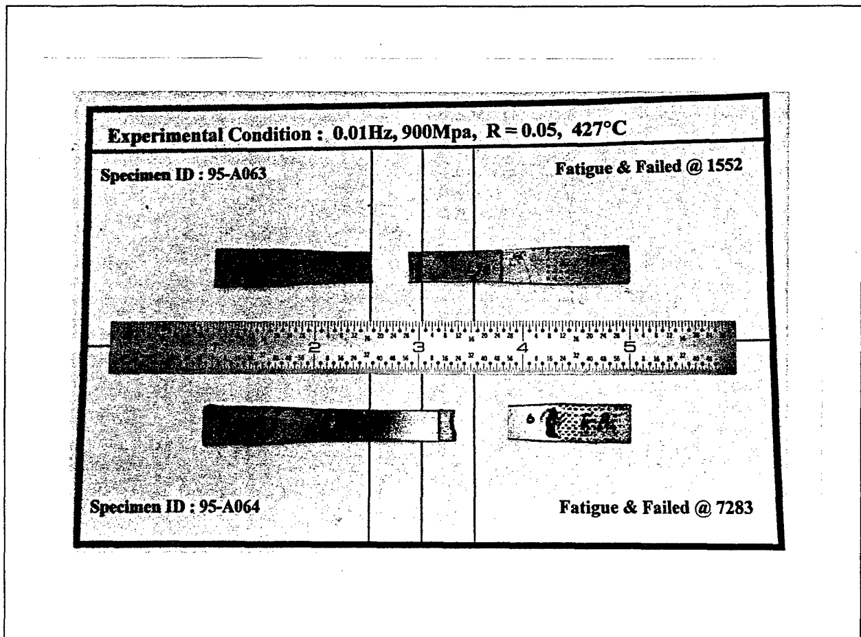
Figure 4.8 Fractured Specimens ( 95-063 & 95-064 )
