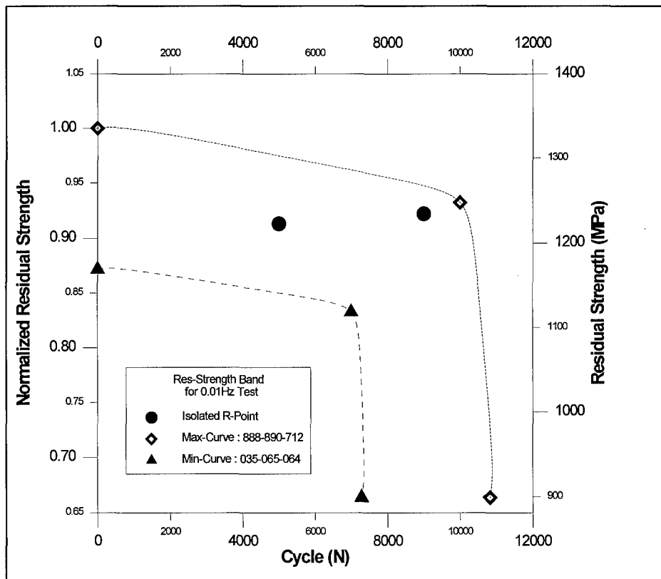
Figure 4.33 Residual Strength vs. Cycles
