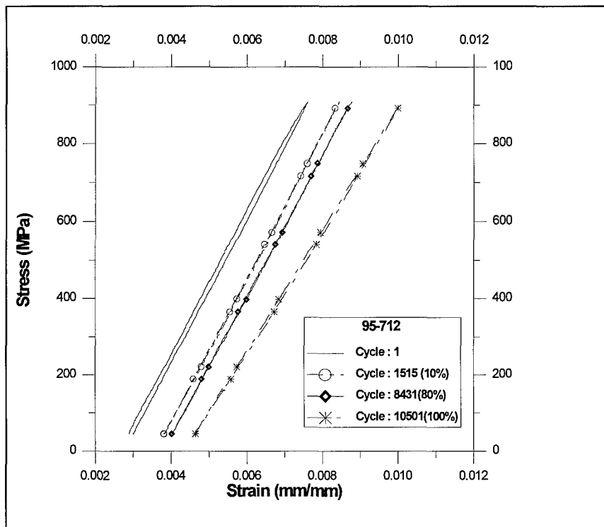
Figure 4.3.2 Stress-Strain Responses of 0.01Hz Test (95-712).
