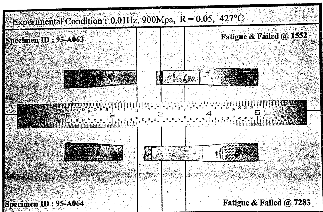
Figure A.6 Specimen Nos. 95-063 and 95-064 (0.01Hz Test)
