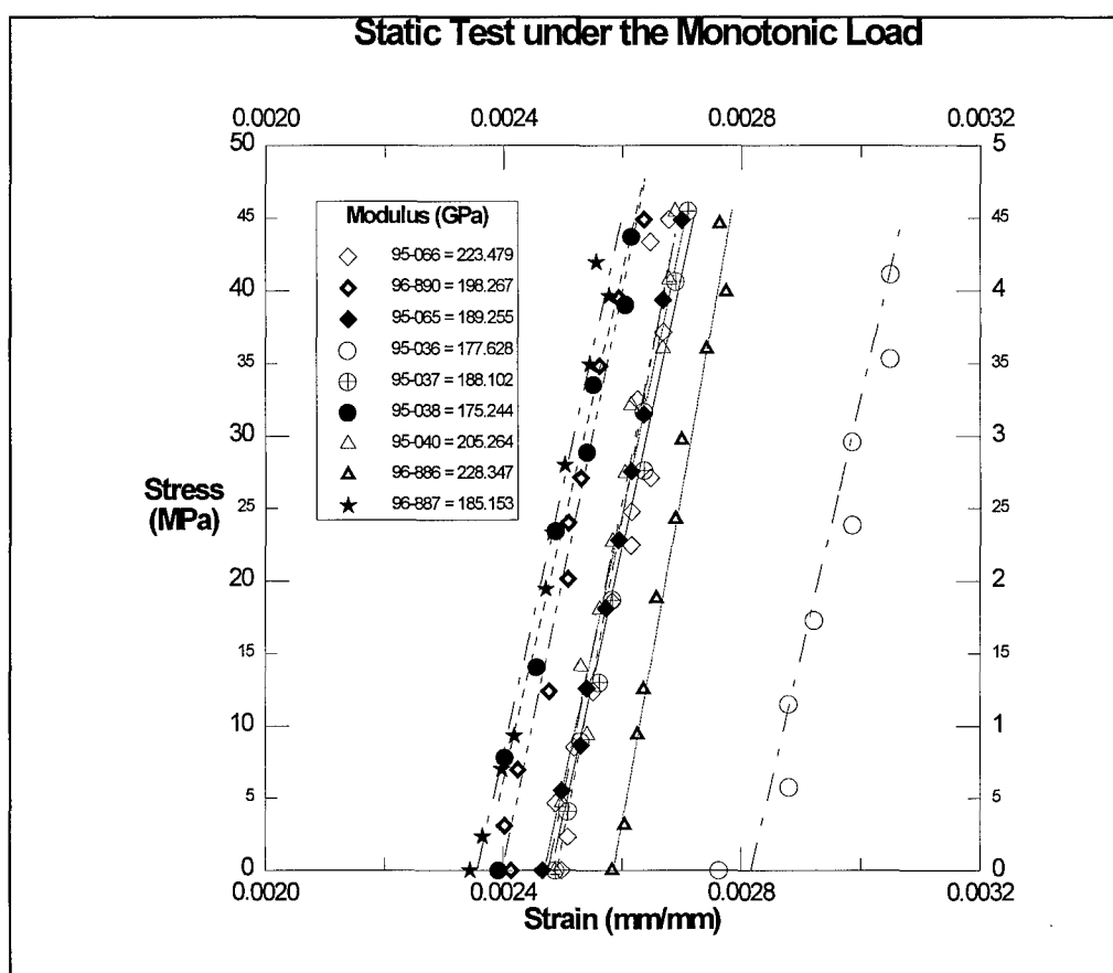
Figure 3.6 Modulus Tests For Three different parent plates
