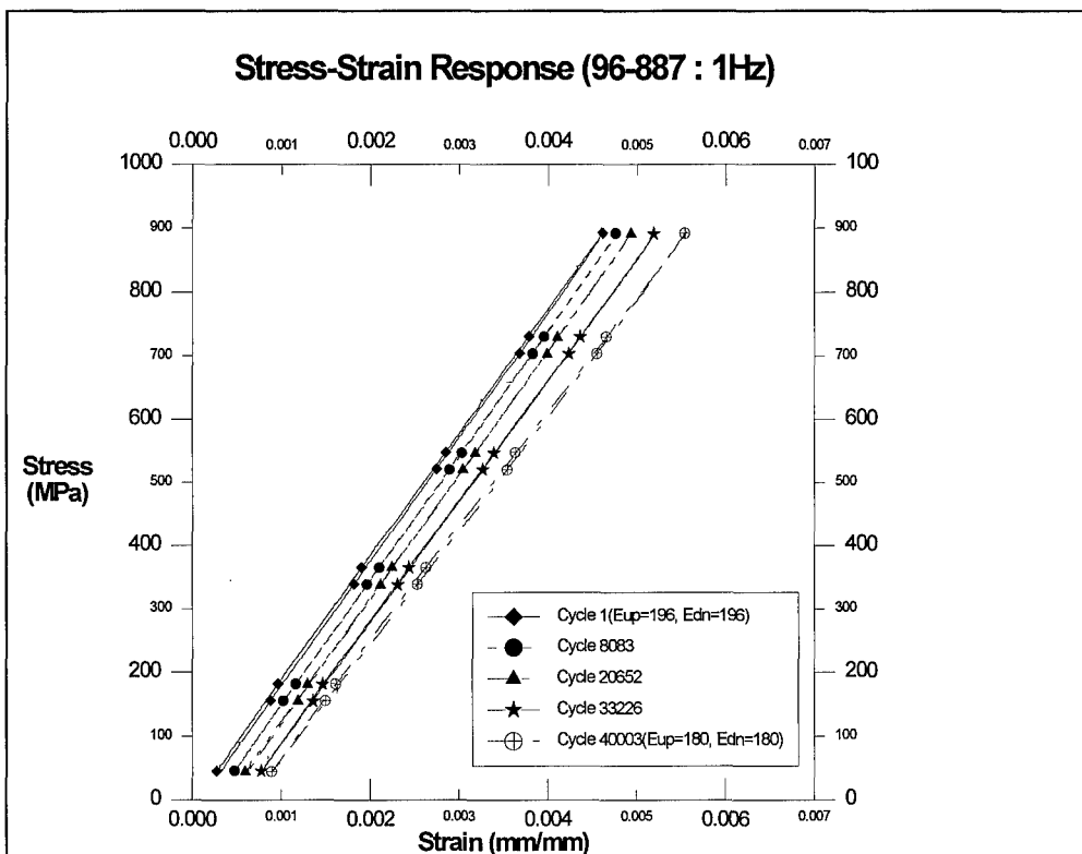
Figure 4.7 Stress-Strain Responses
