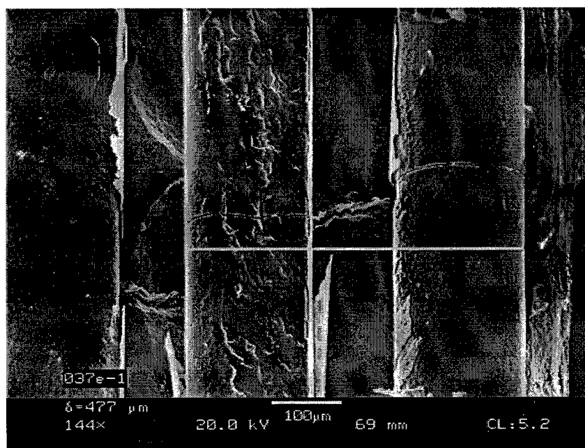
Figure 4.18 Fiber Cracks adjacent the Matrix Cracking
