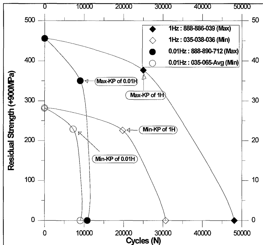
Figure 4.57 The residual strength bands ( \sigma_{\text{Max}} - \sigma_{\text{Res}} ) vs. Cycle.
