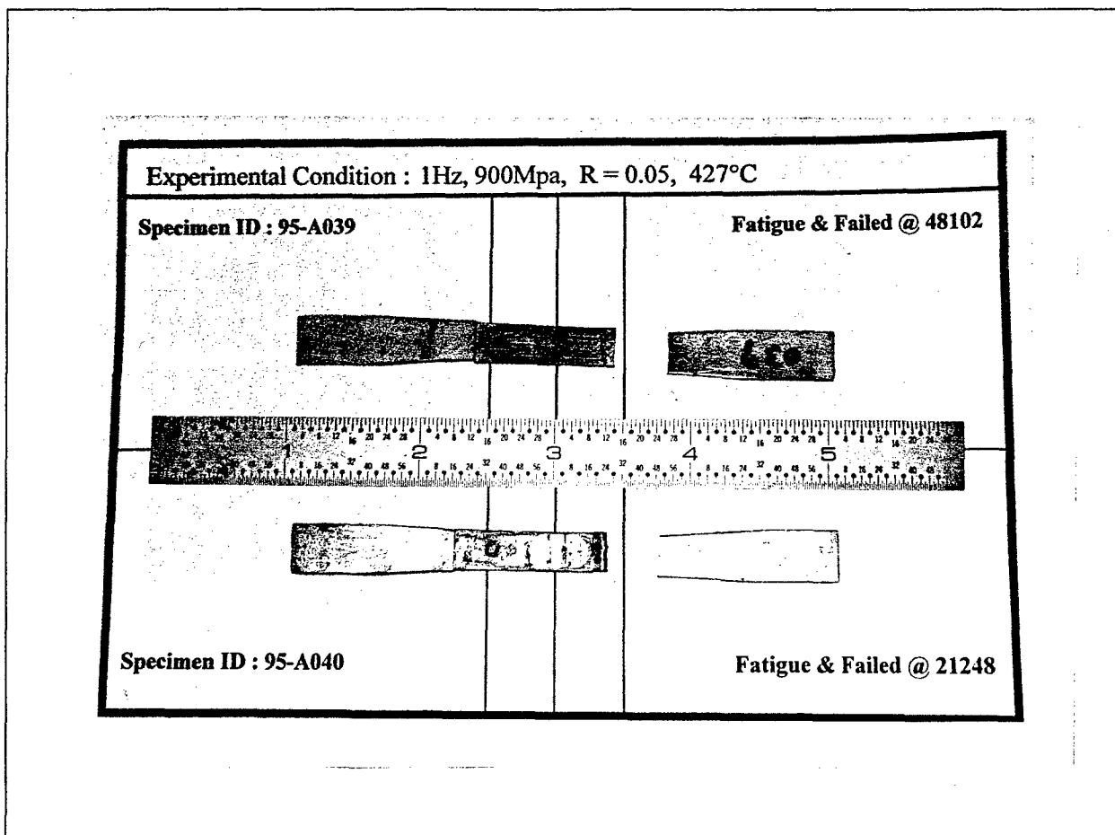
Figure 4.5 Fractured Specimens (95-039 & 95-040)
