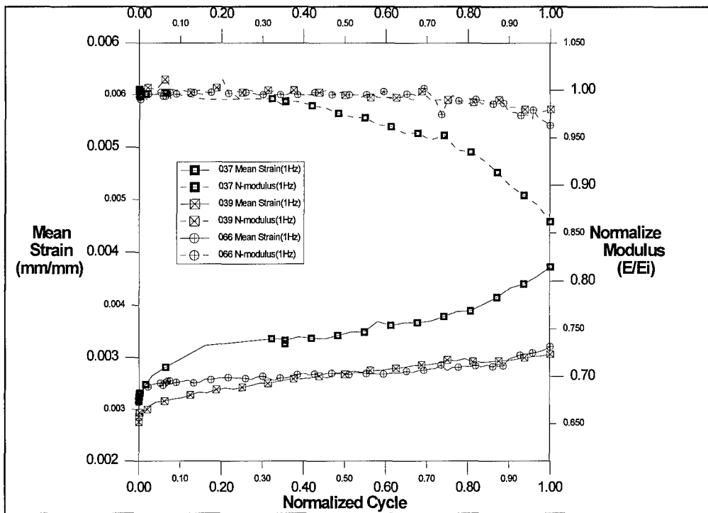
Figure 4.6 Strain and Modulus Responses Comparisons
