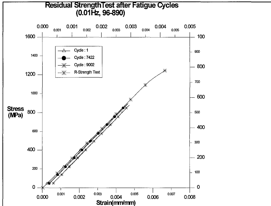
Figure 4.32 Static Test after Fatigue Test
