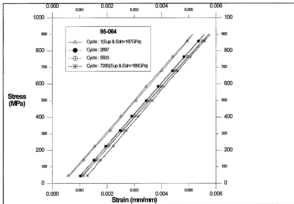
Figure 4.10 Stress-Strain Responses
