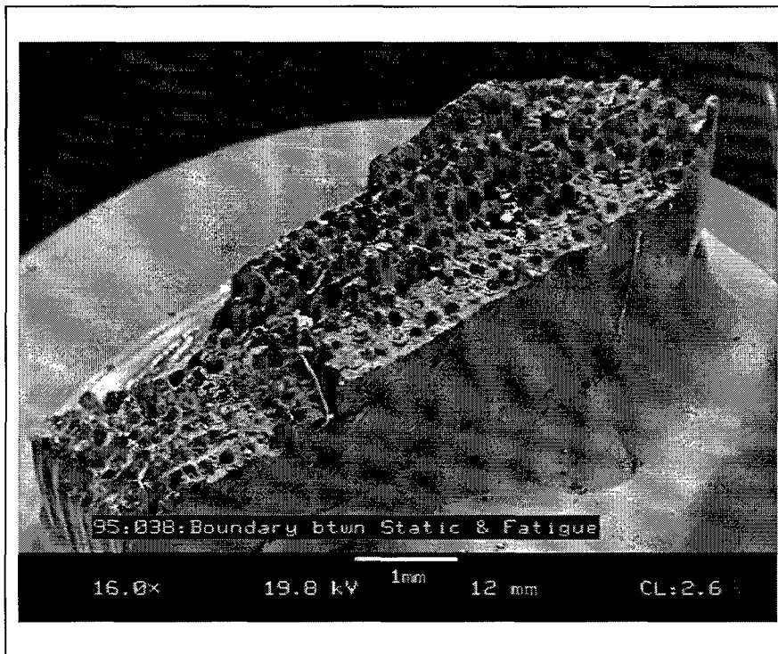
Figure 4.39 Fracture Surface of the R.S. Test at 26% of the Life
