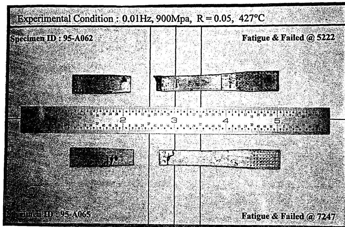
Figure A.7 Specimen Nos. 95-062 and 95-065 (0.01Hz Test)
