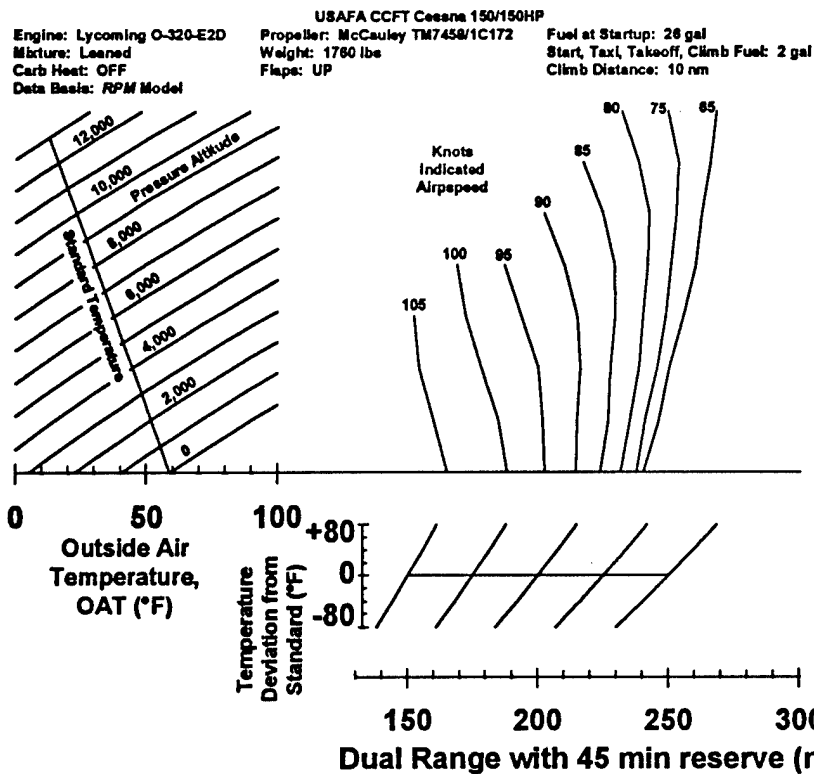
Figure A17 Dual Constant Airspeed Cruise Range Performance With 45 Minute Reserve
