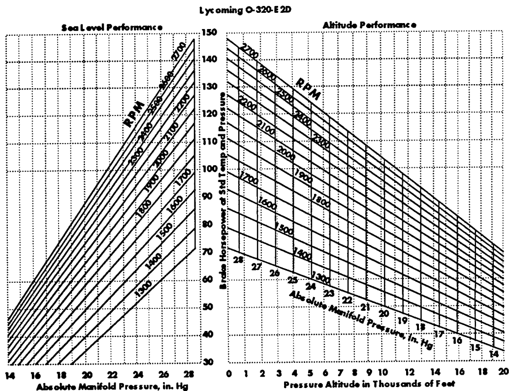
Figure C1 RPM Engine Model For Lycoming O-320-E2D
