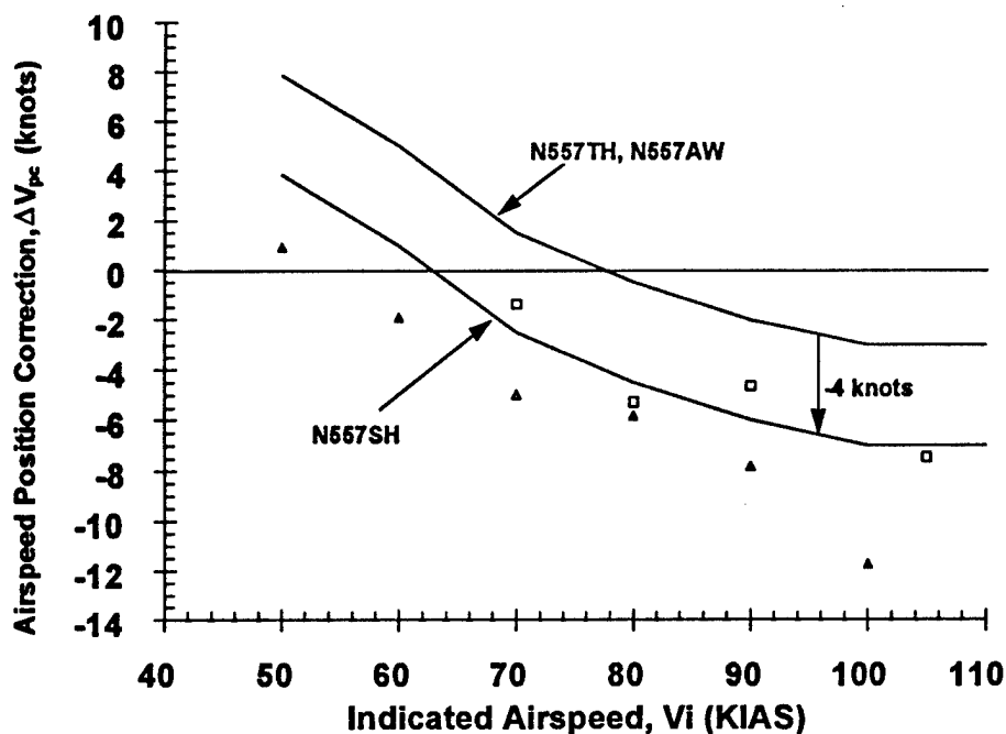
Figure A29 Airspeed Pitot-Static Position Correction, N557SH
