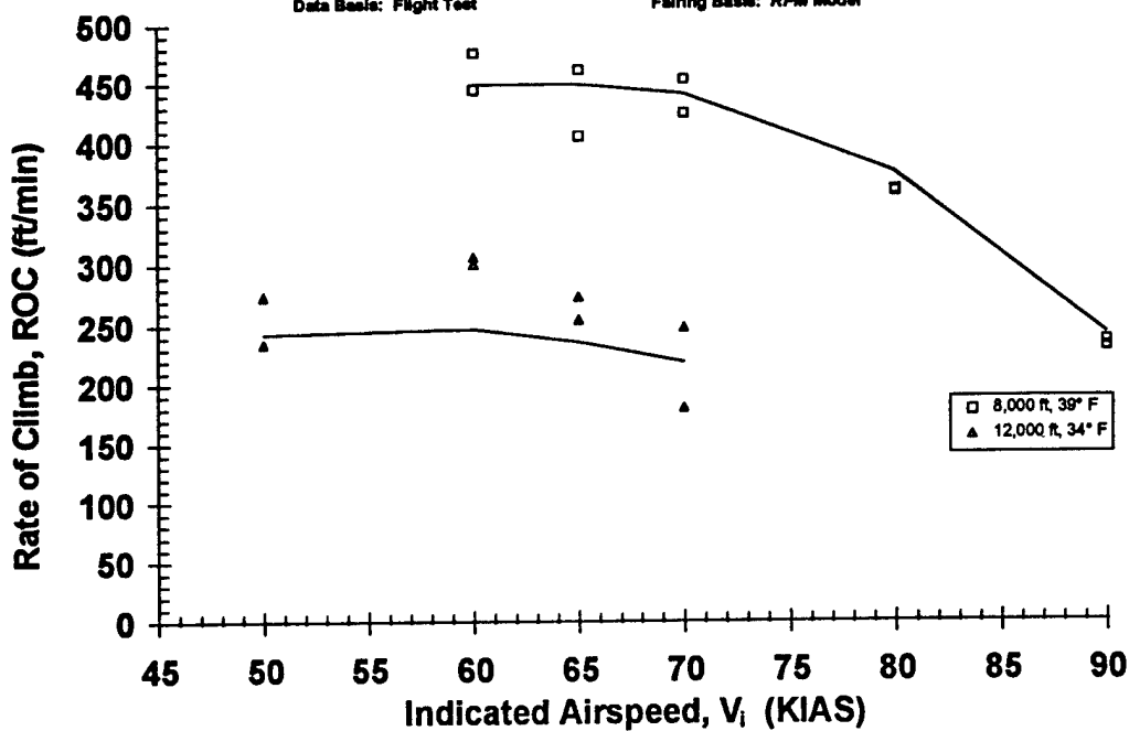
Figure A32 Test Day Rate of Climb Matching
