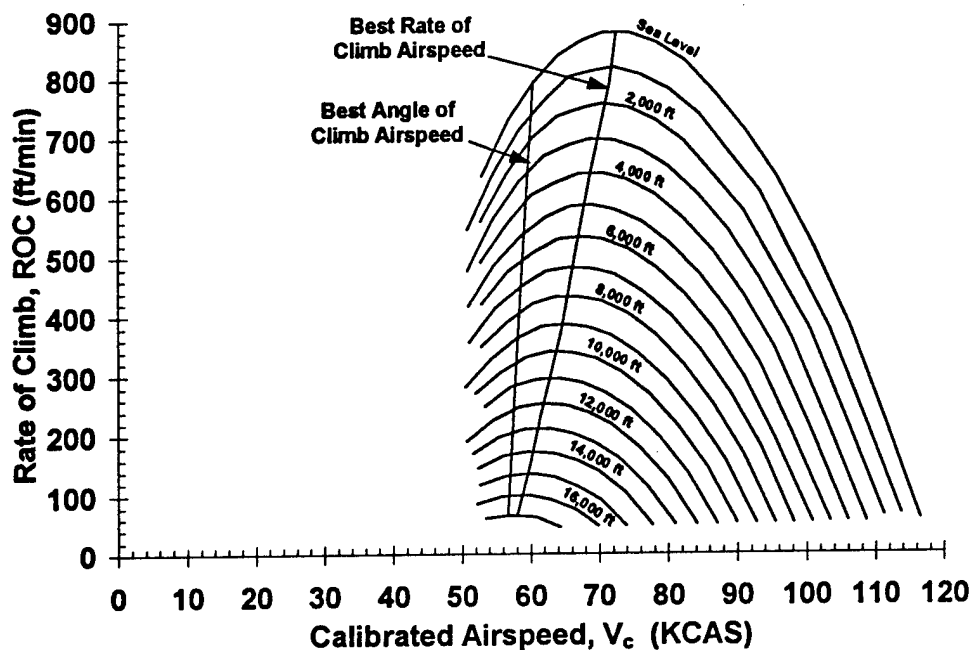
Figure A31 Standard Day Rate of Climb Performance (Calibrated Airspeed)
