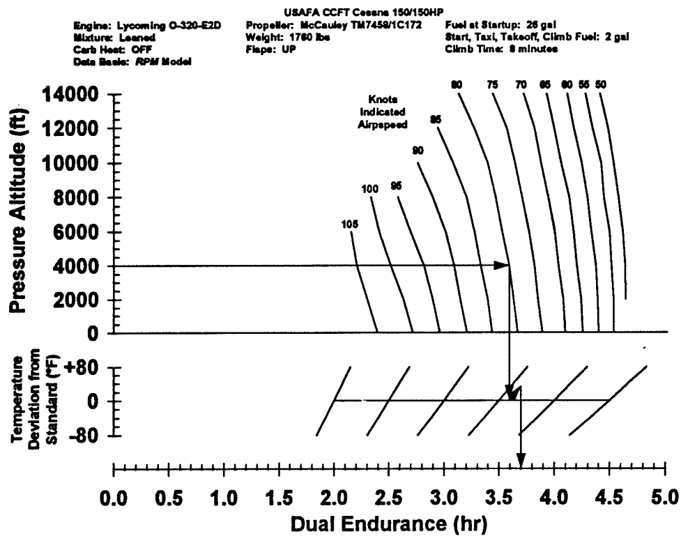
Figure A18 Dual Constant Airspeed Cruise Endurance Performance
