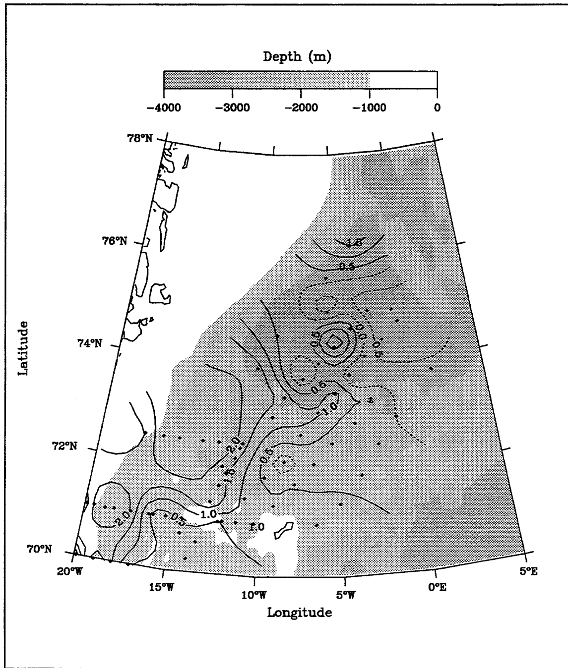
Figure 16. BARTLETT and BJARNI SÆMUNDSSON 90 contours of intermediate temperature maximum (Tmax) (°C). Tmax is associated with the JMatIW of the JMC. The meander, seen in the 0.5°C to 2.0°C isotherms, is similar in shape and location to the surface, both features being affected by the bathymetry. Likewise, the JMC throughput to the GSG is centered at 73°N, best seen in the 0.5°C to 1.5°C isotherms.
