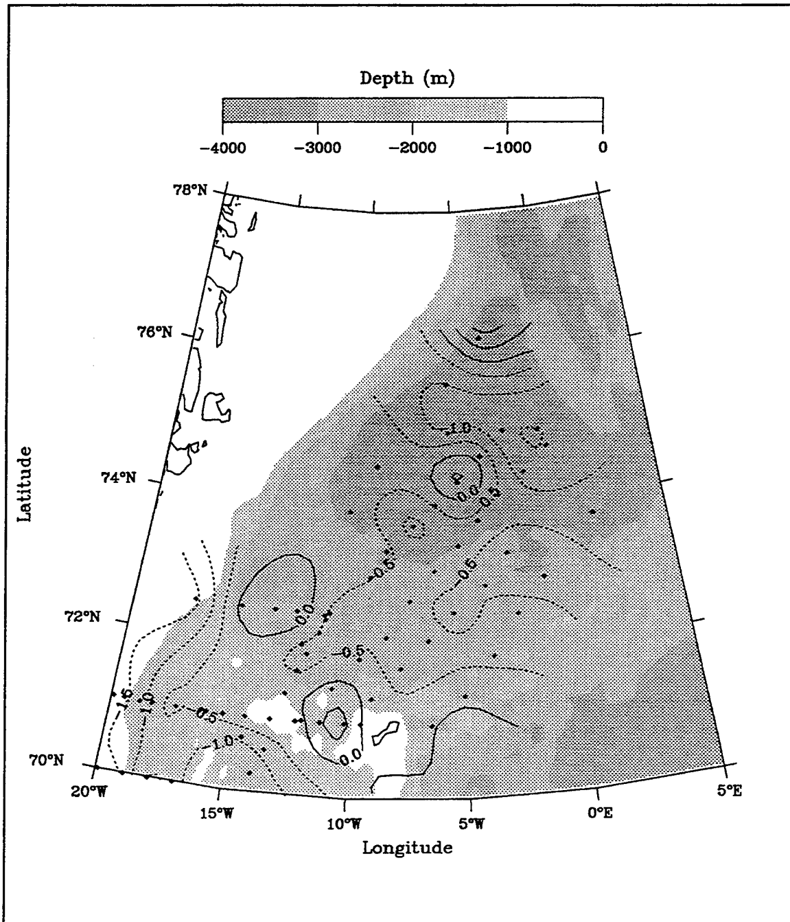
Figure 38. BARTLETT and BJARNI SÆMUNDSSON 90 contours of subsurface temperature minimum (Tmin) (°C). A subsurface temperature minimum occurs between the surface, warmed by insolation and intermediate waters. In the JMC region, Tmin occurs within a shallow subsurface layer of modified GPW termed Jan Mayen Polar Water (JMPW) having a typical Tmin value near -0.5°C.
