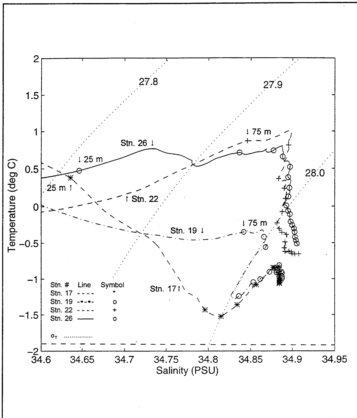
Figure 29. T-S correlations showing Tmax behavior along four stations from Transect B 1990. Two regimes are evident with Stations 22 and 26 representing JMC type waters with a Tmax above 0°C. Stations 17 and 19, at the north end of Transect B, exhibit a Tmax with lower temperatures (< 0°C) and do not mark JMAIw. Data is running-averaged with symbols placed every 50 m. The depth of the first symbol is labeled.
