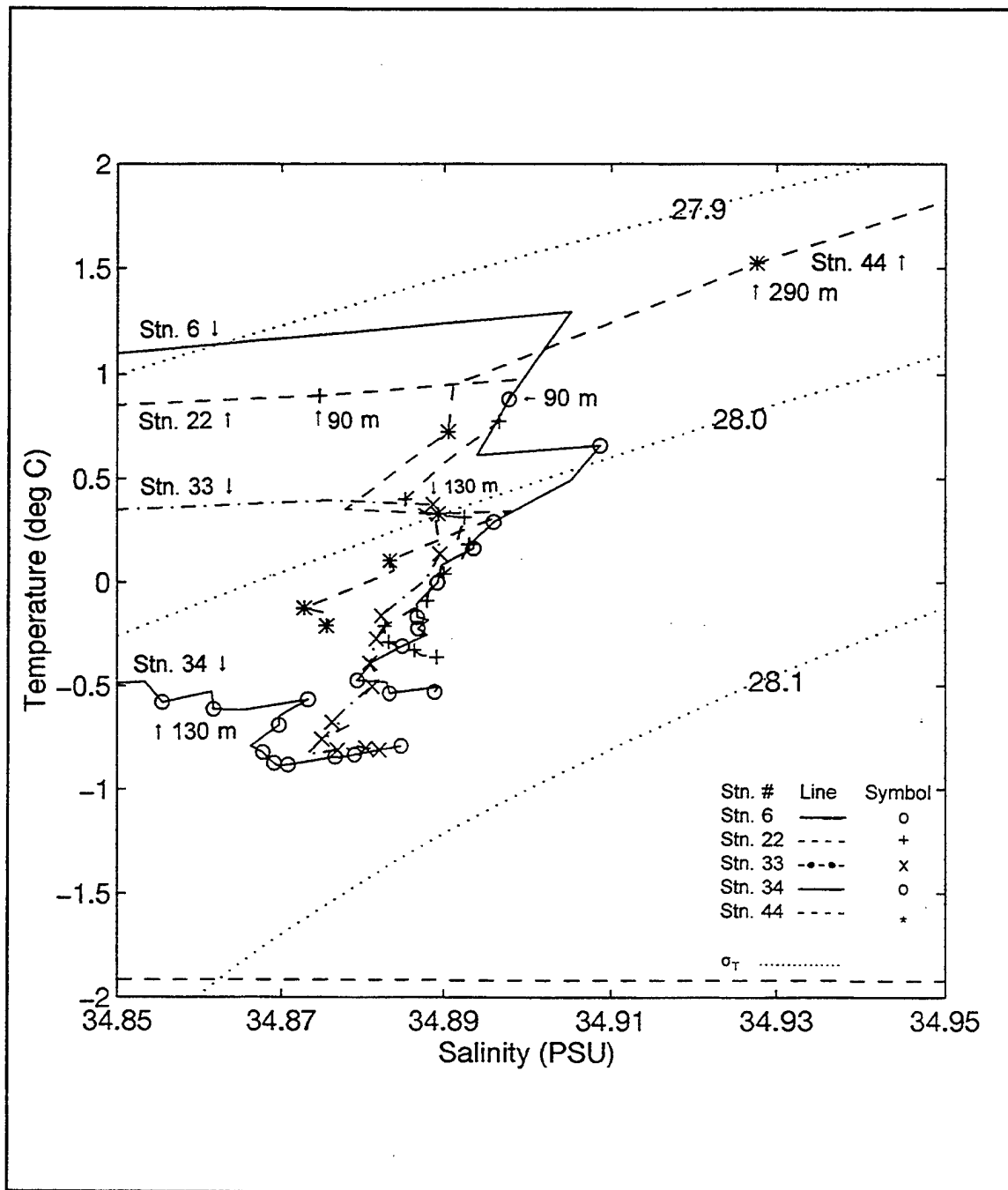
Figure 23. T-S correlations along Transect D showing the progression of T max associated with JMatIW from west to east. Stations 5 and 21 are deleted for clarity. Station 44 is included as an example of water beneath the NAC. Data are block-averaged every 20 m with symbols placed every 40 m. Depth of the first symbol is labeled.
