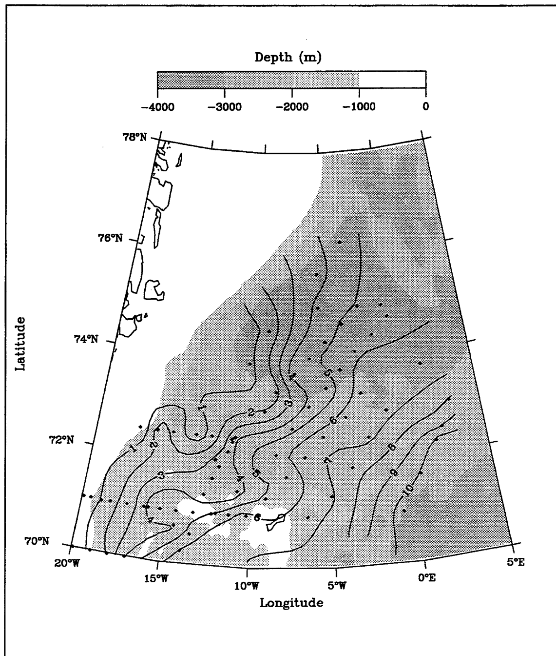
Figure 12. BARTLETT and BJARNI SÆMUNDSSON 90 surface (10 m) temperature (°C). The colder (1°C to 5°C) isotherms bow eastward at about 73°N along the 3000 m isobath which coincides with the base of the slope of the Jan Mayen Fracture Zone (JMFZ) to the south. Temperatures to 10°C occur over the Lofoten Basin where the warm NAtSW of the NAC is encountered.
