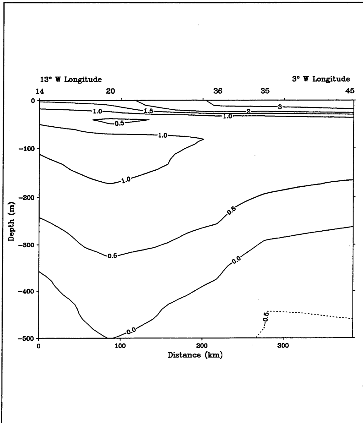
Figure 27. BARTLETT 89 temperature along Transect D ( ^{\circ}\text{C} ). This west to east section represents the region of greatest throughput of JMA tl W eastward during 1989 and is south of the 1990 position by about 100 km. JMA tl W, bounded by the 0^{\circ}\text{C} isotherm, encompasses a larger area compared to 1990. As is typical, T_{\text{max}} is centered at 100 m.
