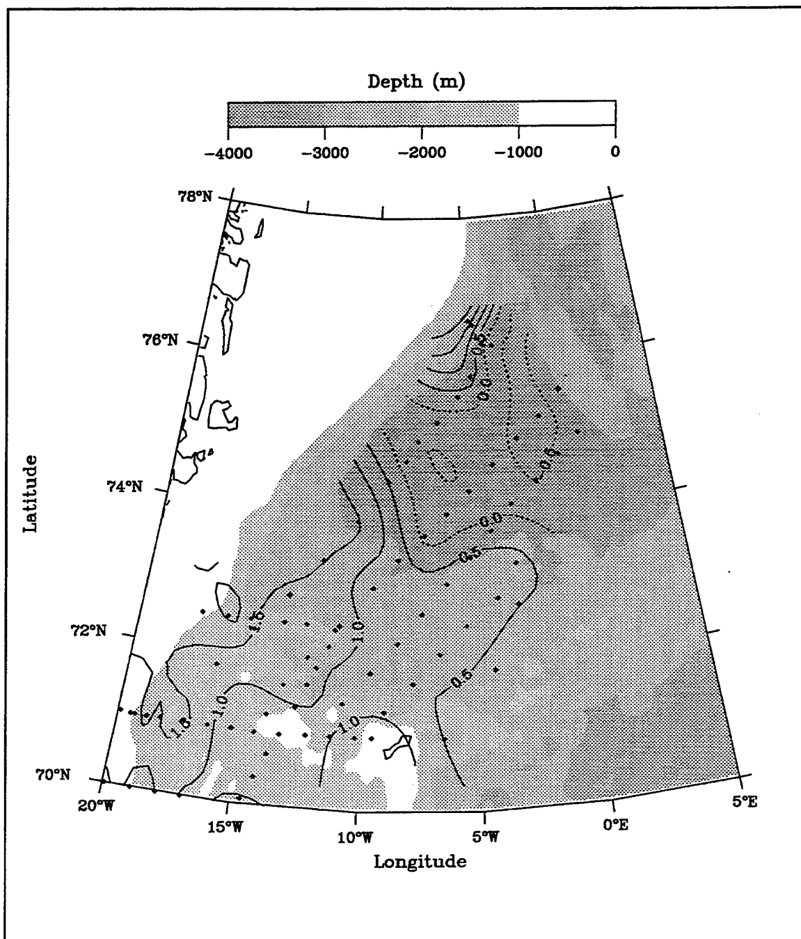
Figure 19. BARTLETT and BJARNI SÆMUNDSSON 89 contours of intermediate temperature maximum ( T_{max} ) ( ^{\circ}\text{C} ). Similar to 1990, the JMC is evident in the eastward protrusion of the 0.5^{\circ}\text{C} isotherm. There is a lack of eddy-like features compared to 1990.
