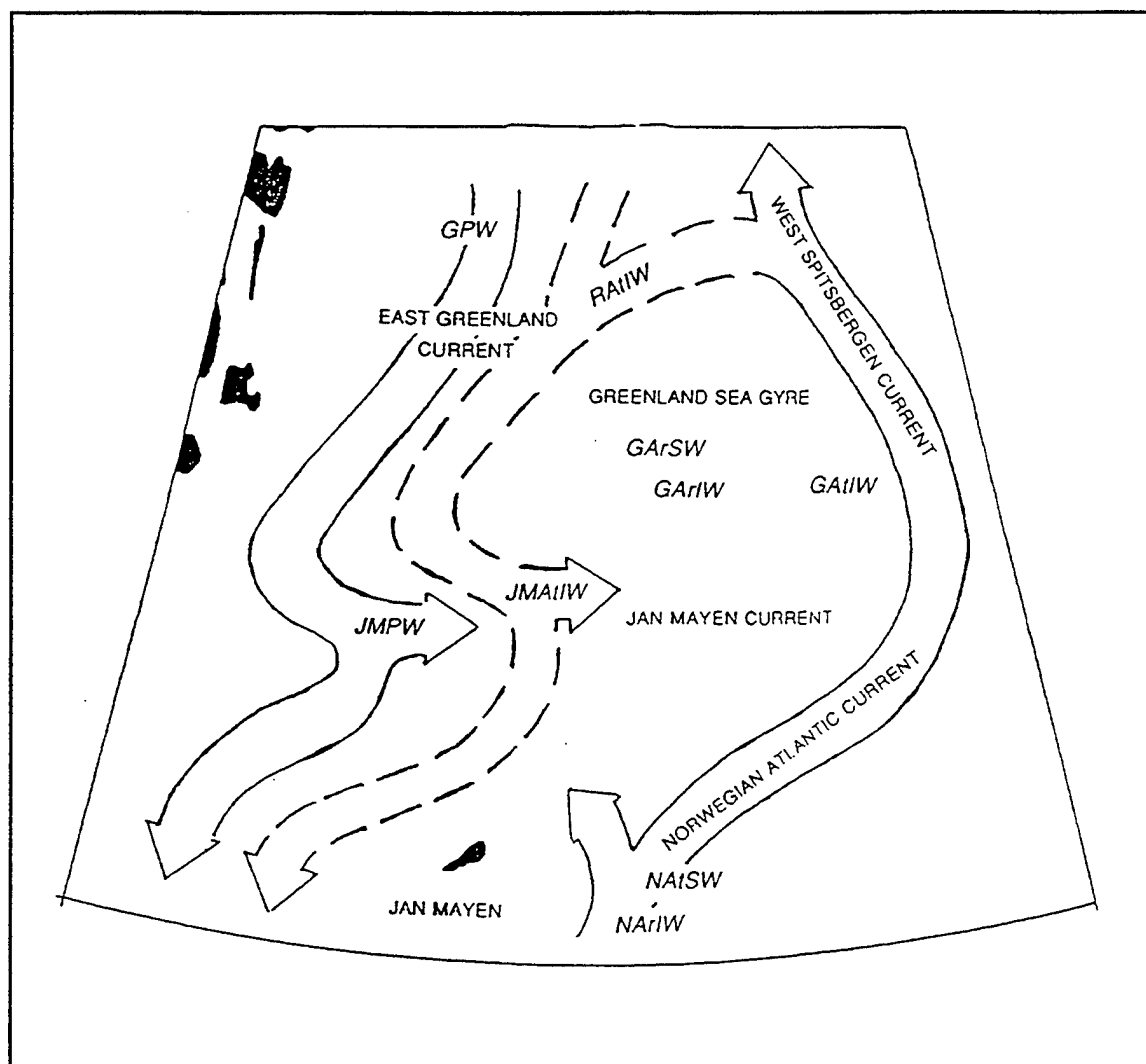
Figure 6. Greenland-Norwegian Sea surface and intermediate water mass circulation schematic. In the north, the East Greenland Current (EGC) carries surface Greenland Polar Water (GPW) from the Arctic Ocean in to the region; similarly in the south, the Norwegian Atlantic Current (NAC) carries in Norwegian Atlantic Surface Water (NAtSW) and Norwegian Arctic Intermediate Water (NArIW). NAtSW sinks isopycnally in the West Spitsbergen Current (WSC) to supply intermediate water to the Arctic Ocean via Fram Strait, the EGC as Return Atlantic Intermediate Water (RAtIW), and directly to the Greenland Sea from the east as Greenland Atlantic Intermediate Water (GAtIW). The Jan Mayen Current (JMC) contains not only throughput to the east but also a large meander in the EGC. The cyclonic Greenland Sea Gyre (GSG) consists of a mixture of waters from the surrounding circulations. Refer to Table 1 for complete water mass descriptions (from Blythe, 1990 ).
