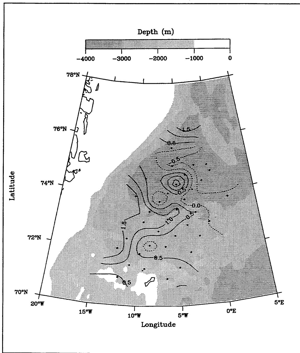
Appendix B, Figure 6. BARTLETT 90 contours of intermediate temperature maximum (T max ) (°C). The BJARNI SÆMUNDSSON 90 data has not been combined with BARTLETT data. Comparison with Figure 16 allows the reader to assess any distortions caused by combining the two data sets.
