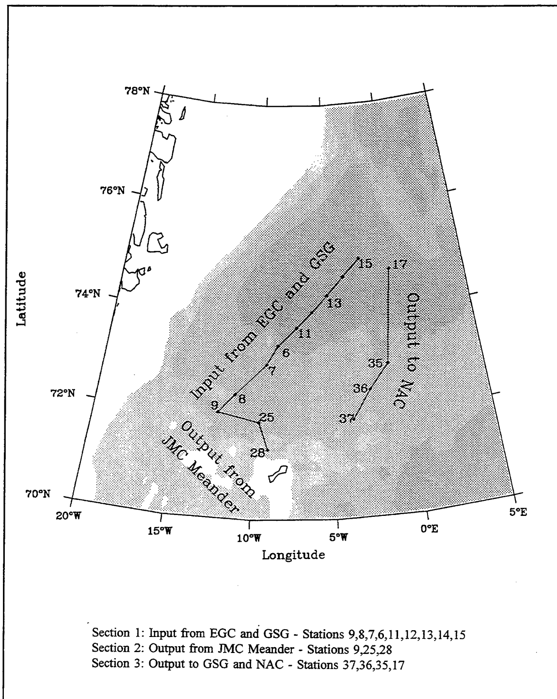
Figure 46. BARTLETT 90 station sections used to determine baroclinic transports. Selections are based on sets of stations located roughly normal to dynamic height contours.
