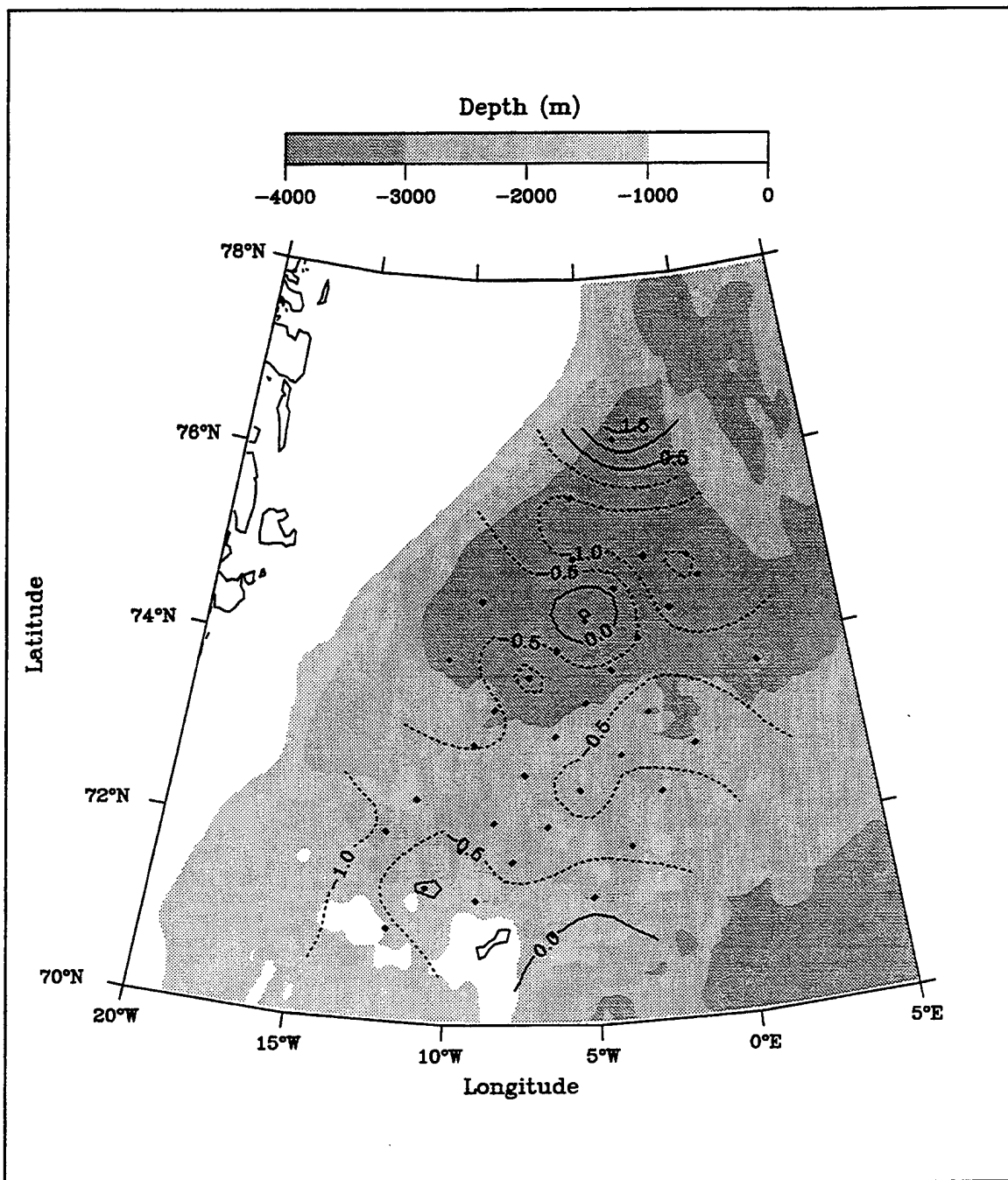
Appendix B, Figure 9. BARTLETT 90 contours of subsurface temperature minimum (T min ) (°C). The BJARNI SÆMUNDSSON 90 data has not been combined with BARTLETT data. Comparison with Figure 38 allows the reader to assess any distortions caused by combining the two data sets.
