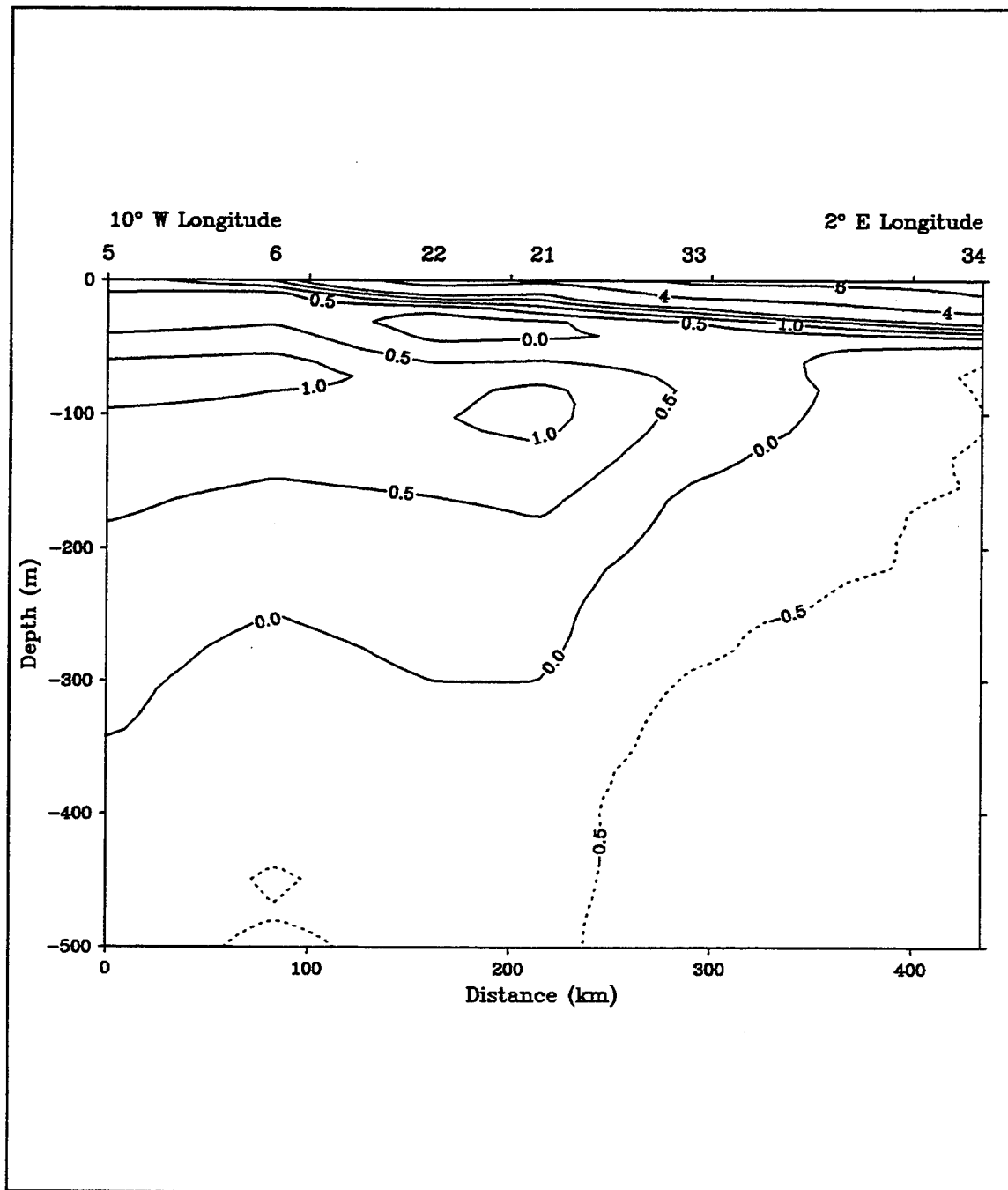
Figure 24. BARTLETT 90 temperature along Transect D ( ^{\circ}\text{C} ). This west to east section shows the course of JMatIW as it moves eastward across the southern portion of the GSG. Tmax is found close to 100 m and deepens to the east. JMatIW, bounded by the 0^{\circ}\text{C} isotherm, rides up over the colder GArIW to the east. This doming is associated with the cyclonic rotation of the GSG.
