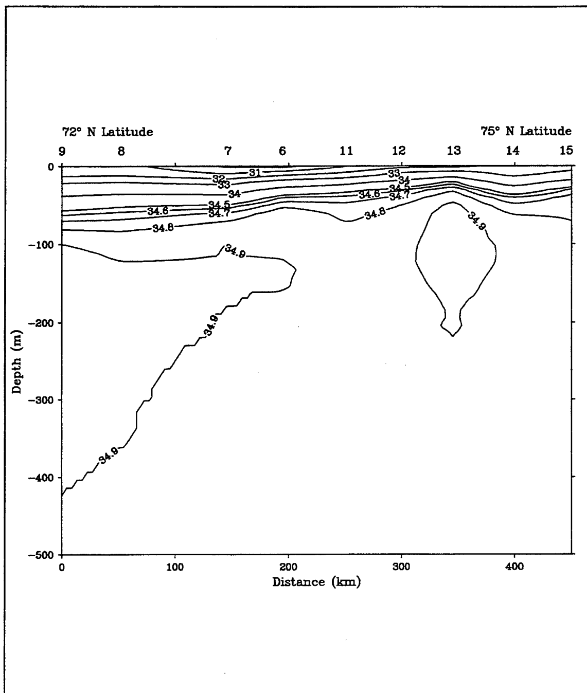
Figure 35. BARTLETT 90 salinity along Transect A (PSU). As in Transect B, salinities exceeding 34.9 PSU indicate JMatIW from Station 6 southward. A similar salinity is present in the eddy at Station 13.
