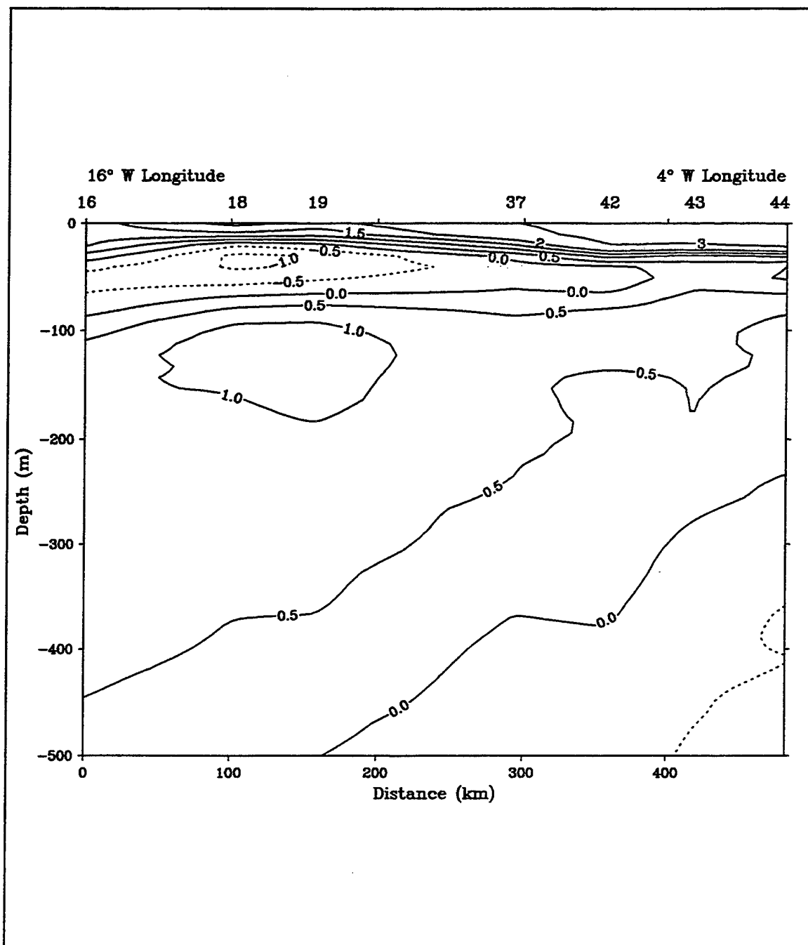
Figure 44. BARTLETT 89 temperature along Transect C ( ^{\circ}\text{C} ). This west to east section is similar in position to 1990 and exhibits the maximum expression of JMW from 1989 data. Similar to 1990, JMW is centered at 50 m in a shallow layer with temperature less than 0^{\circ}\text{C} . This section, which is displaced to the west relative to Transect C for 1990, exhibits colder subsurface temperatures in the west due to closer proximity to the EGC and did not cross into the NAC in the east.
