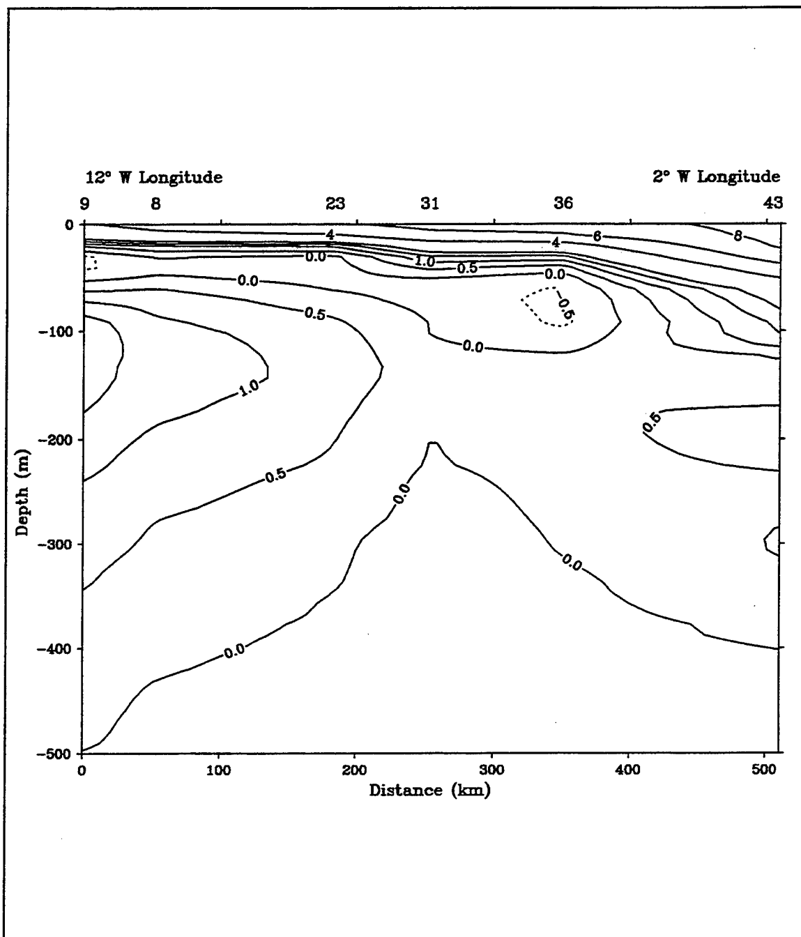
Figure 42. BARTLETT 90 temperature along Transect C (°C). This west to east trending section at about 72°N shows the maximum expression of JMPW for 1990 in a subsurface layer from 50 to 75 m with temperatures less than 0°C. JMPW deepens to the east as GSG is encountered.
