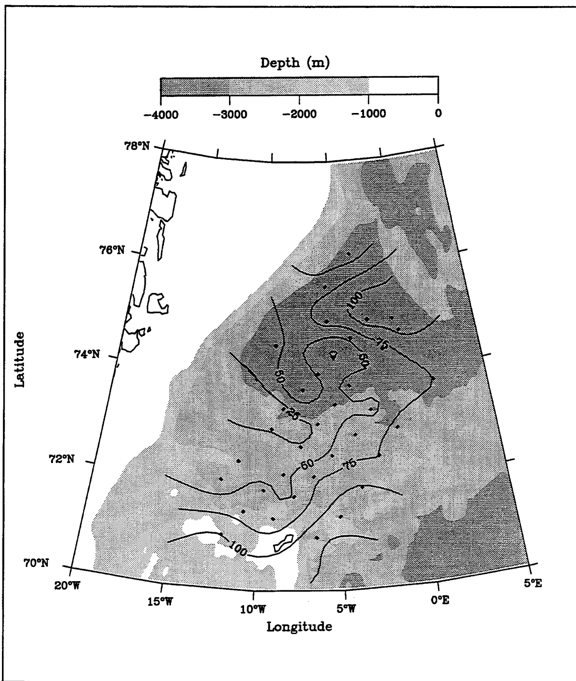
Appendix B, Figure 10. BARTLETT 90 depth of subsurface temperature minimum ( T_{min} ) (m). The BJARNI SÆMUNDSSON 90 data has not been combined with BARTLETT data. Comparison with Figure 39 allows the reader to assess any distortions caused by combining the two data sets.
