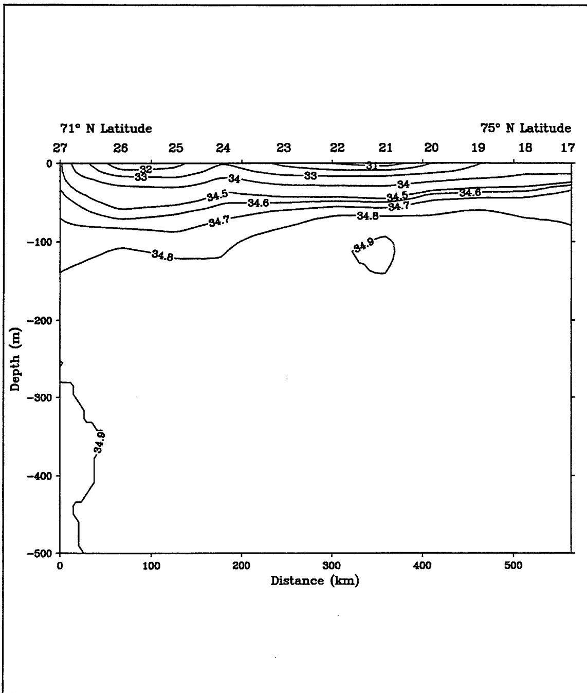
Figure 31. BARTLETT 90 salinity along Transect B (PSU). The core of JMA 1 W is again seen at Station 21. Salinities corresponding to JMA 1 W typically exceed 34.9 PSU. The lower salinities associated with the meander are present to the south.
