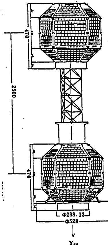
Fig.4 Exterior Structure of Miniature Satellite
