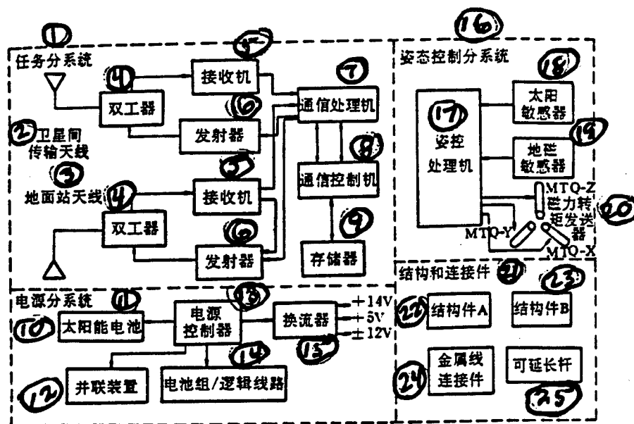
Fig.3 Satellite System Block Diagram
