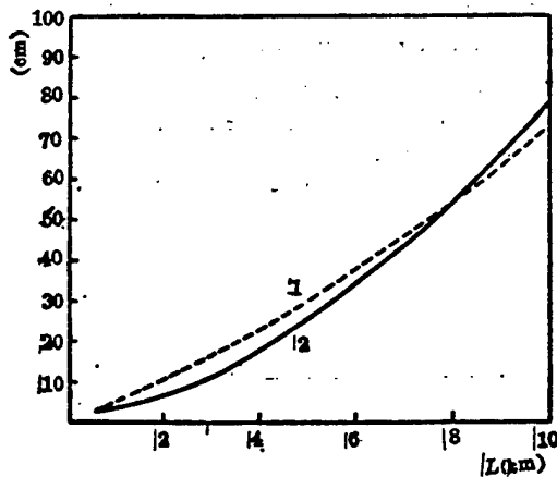
Fig. 5 Effective radius r_m vs field range L for different wavelength C_n^2 = 10^{-14} \text{ m}^{-2/3} , a = 2.5 \text{ cm} 1— \lambda = 3.8 \mu\text{m} ; 2— \lambda = 1.06 \mu\text{m}
