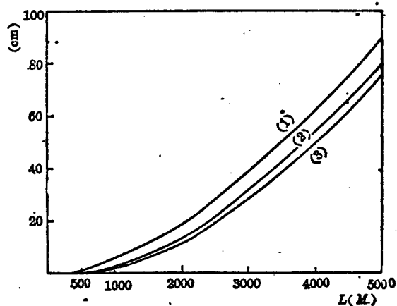
Fig. 6 Relative effective radius r_m vs field range L for different aperture size C_n^2 = 10^{-13} \text{ m}^{-2/3} , \lambda = 1.06 \mu\text{m} 1— a = 2.5 \text{ cm} ; 2— a = 10 \text{ cm} ; 3— a = 15 \text{ cm}
