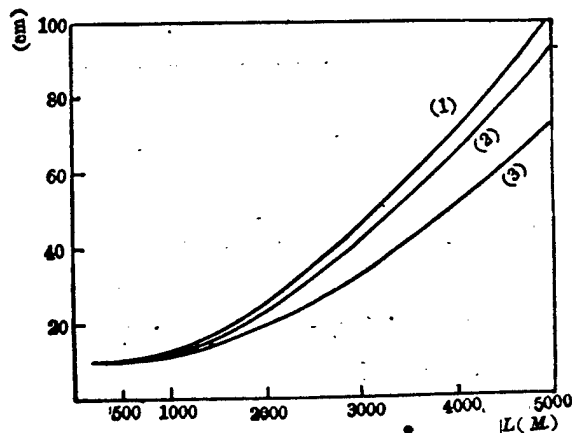
Fig. 4 Effective radius r_m vs field range L for different wavelength
