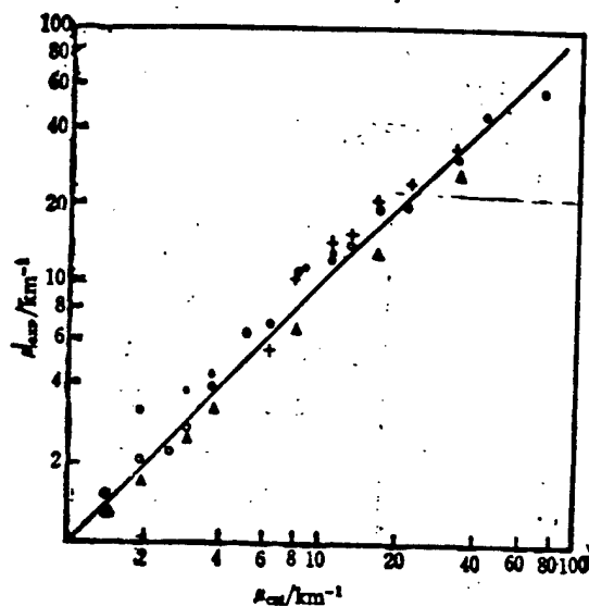
Fig. 3 Comparison of theoretical and experimental attenuation coefficient. O—present measurement \Delta —Grimm (2) ●—Deng Benda et al., 1968, Beijing +—Wang Dinghua et al., 1975, Qingdao
