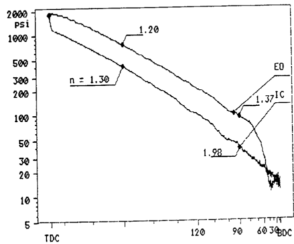
Figure E.8 Log Pressure vs. Log Volume CC1812P1.DAT
