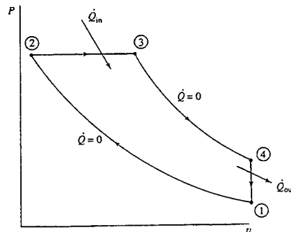
Figure 4.6 Theoretical Diesel PV diagram [Ref 16]
