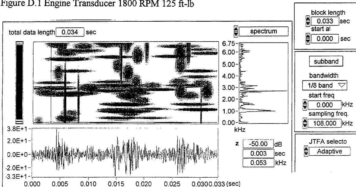
Figure D.2 Engine Transducer 1800 RPM 125 ft-lb
