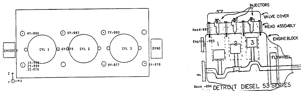
Figure 3.5 Accelerometer Locations (Sensor number, Axis of measure, Serial Number)
