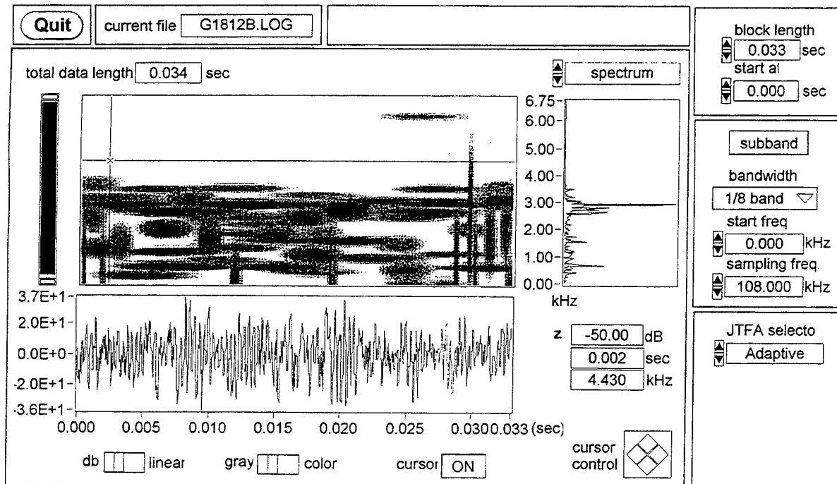
Figure D.23 Engine Base Transducer 1800 RPM 125 ft-lb
