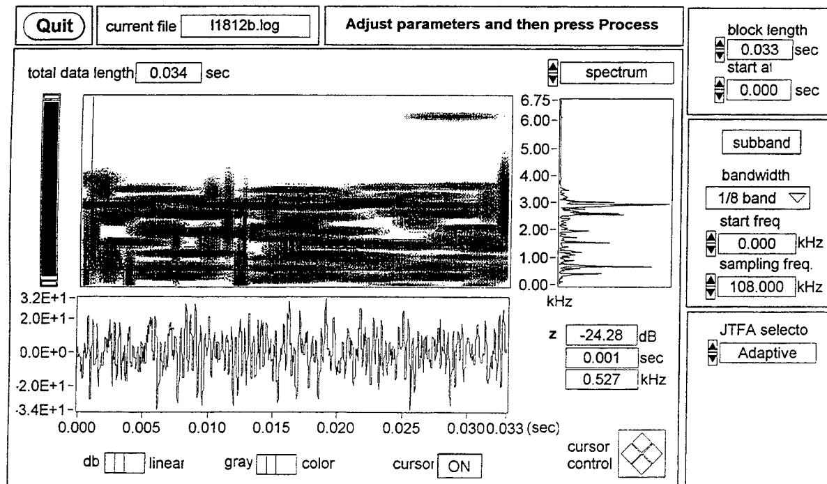
Figure D.43 Engine Base Transducer 1800 RPM 125 ft-lb
