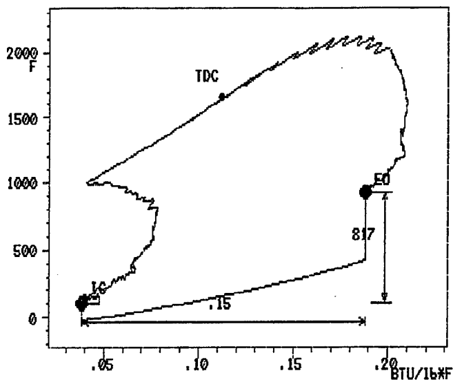
Figure 4.8 Temperature vs. Entropy
