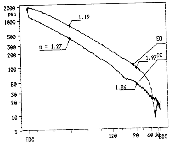
Figure E.4 Log Pressure vs. Log Volume BB1812P1.DAT
