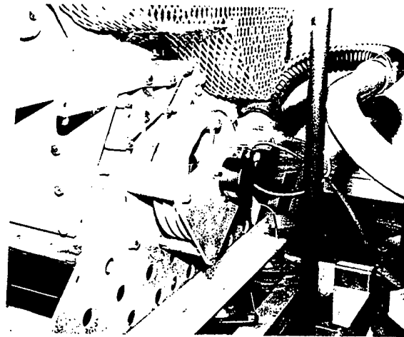
Figure 3.2 Heidenhain 3600 Count Optical Encoder and Mounting Bracket
