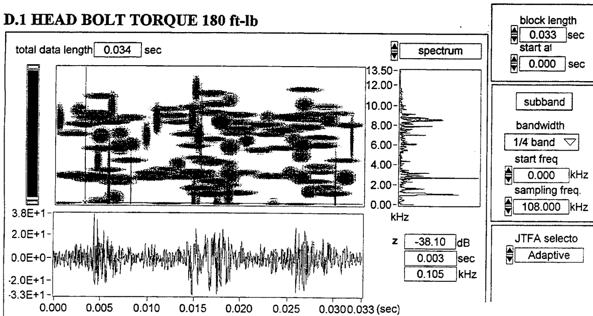
Figure D.1 Engine Transducer 1800 RPM 125 ft-lb
