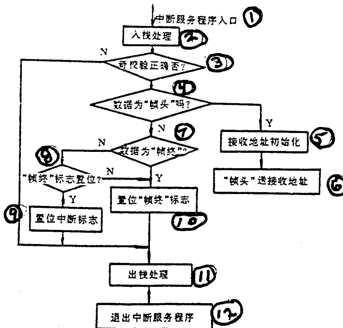
Fig.4 Service Suspension Program Flow Chart (1) Service Suspension Program Input (2) Input to Storage for Processing (3) Odd Parity Correct of Not? (4) Is Data "Frame Header"? (5) Received Address Initialization (6) "Frame Header" Send and Receive Addresses (7) Is Data "Frame End"? (8) "Frame End" Index in Position? (9) Suspension Index Set (10) "Frame End" Index In Position (11) Leave Storage for Processing (12) Leave Service Suspension Program
