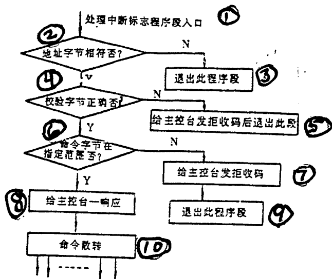
Fig.5 Flow Chart for Processing Suspension Index Program Sections (1) Process Suspension Index Program Section Input (2) Address Groups Match or Not? (3) Leave This Program Section. (4) Group Verification Correct or Not? (5) After Sending Transmission Refused Code to Main Control Unit, Leave This Section. (6) Command Group Within Specified Range or Not? (7) Transmit Reception Refused Code to Main Control Unit. (8) Give a Response to Main Control Unit. (9) Leave This Program Section. (10) Command Dissemination
