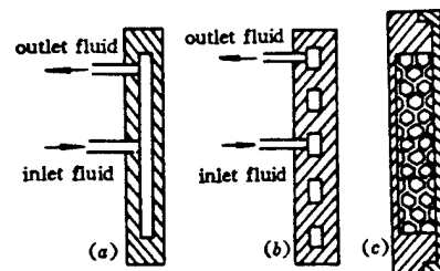
Fig. 2. (a) cavity-structure mirror (b) annular-channel mirror (c) new structure type mirror
