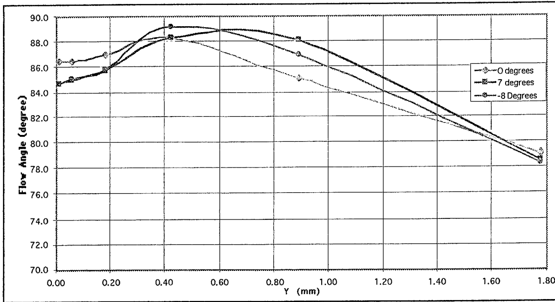
Figure 20. A radial survey through the laser blank at a Prandtl number of 0.9620
