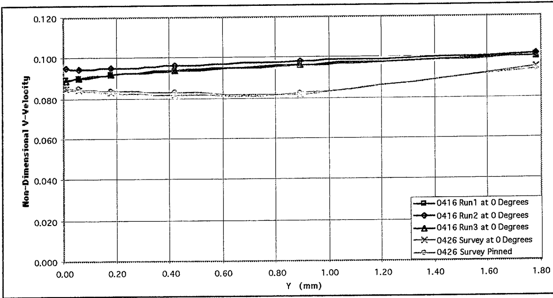
Figure 15b. A radial survey through the laser blank at a Prandtl number of 0.9054
