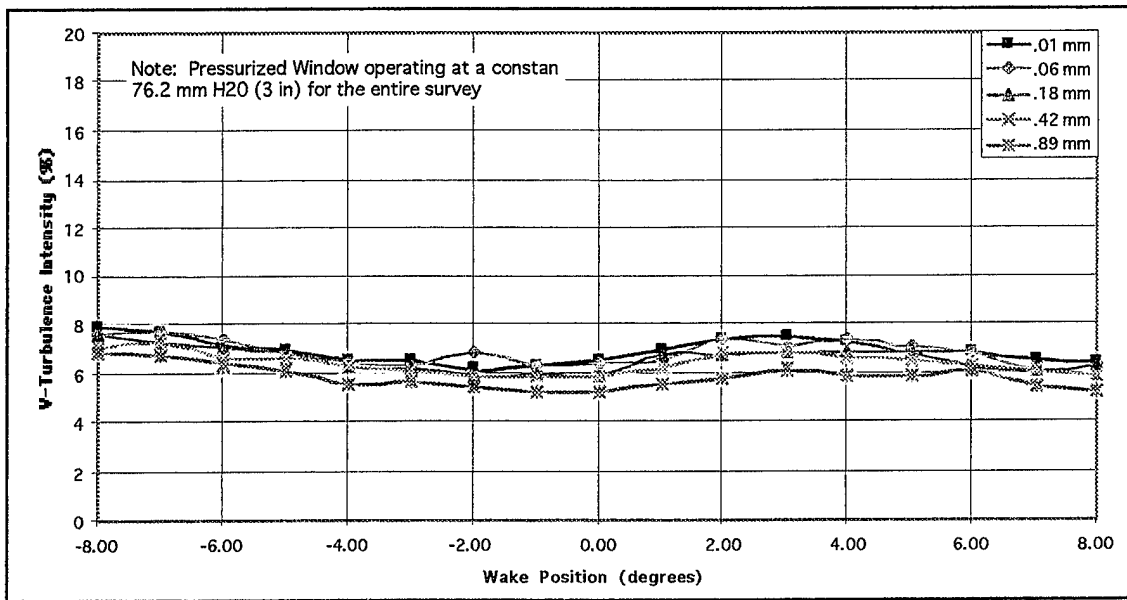
Figure 34b. A circumferential survey through the pressurized LDV window at a Pr at of 0.9620
