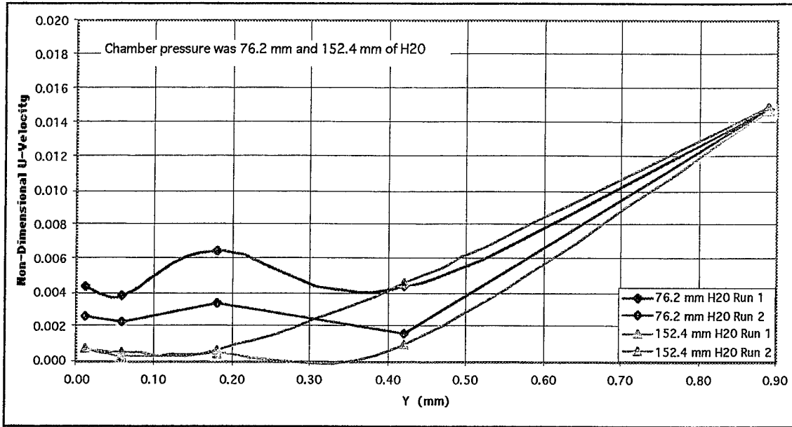
Figure G1a. A radial survey through the pressurized window at a Pr at of 0.9054
