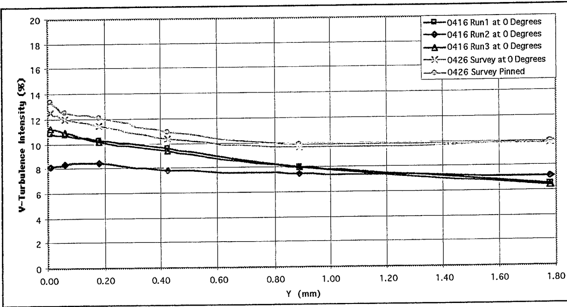
Figure 16b. A radial survey through the laser blank at a Prandtl number of 0.9054
