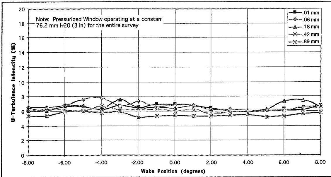
Figure 34a. A circumferential survey through the pressurized LDV window at a Pr at of 0.9620
