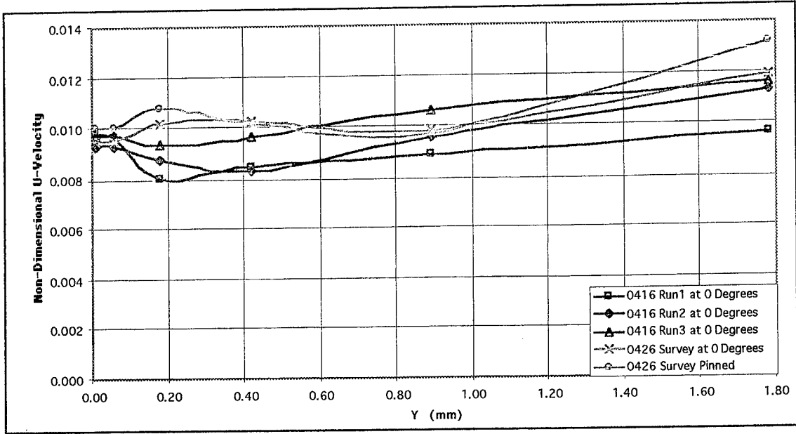
Figure 15a. A radial survey through the laser blank at a Prandtl number of 0.9054
