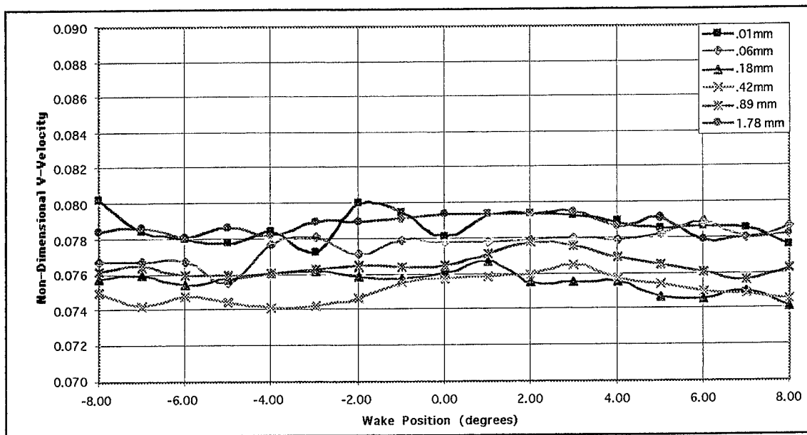
Figure 21b. A circumferential survey through the laser blank at a Prandtl of 0.9620
