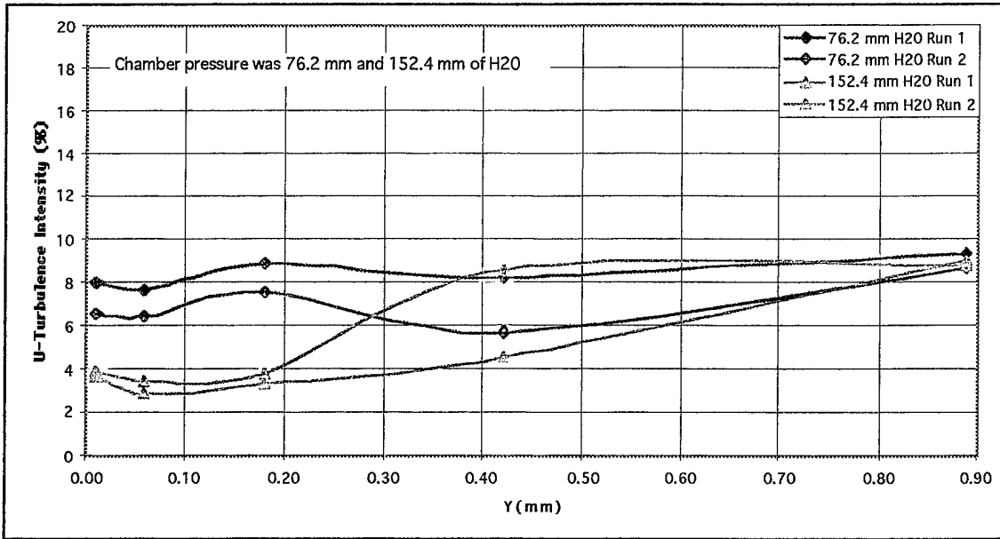
Figure G2a. A radial survey through the pressurized window at a Prandtl of 0.9054
