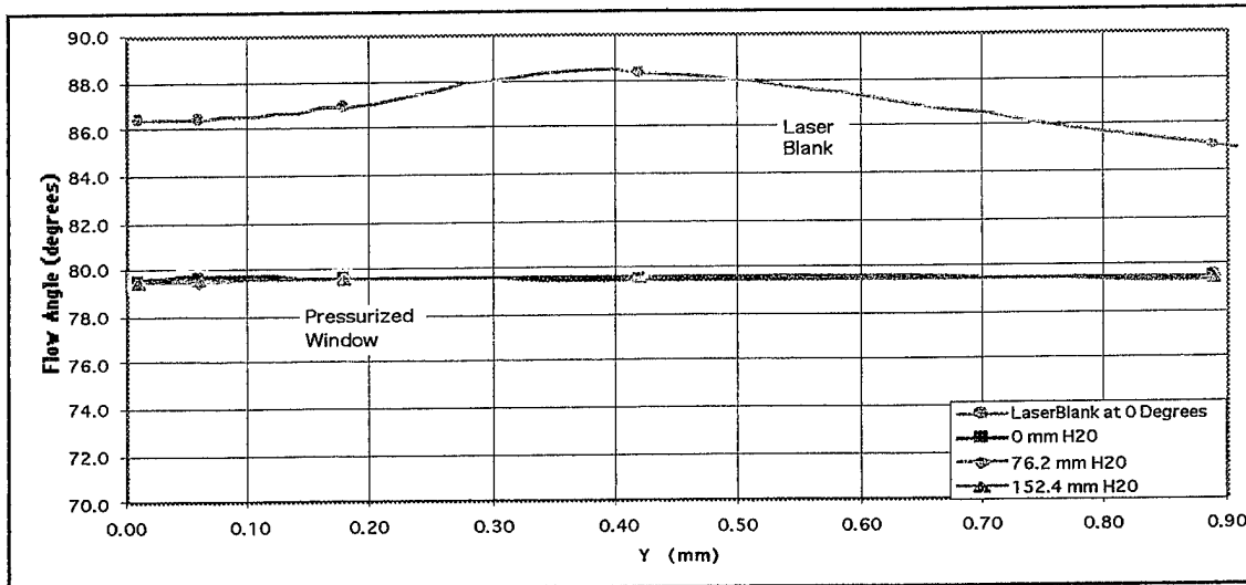
Figure 29. Comparisons of radial surveys using the laser blank and pressurized LDV window at a Pr of 0.9620
