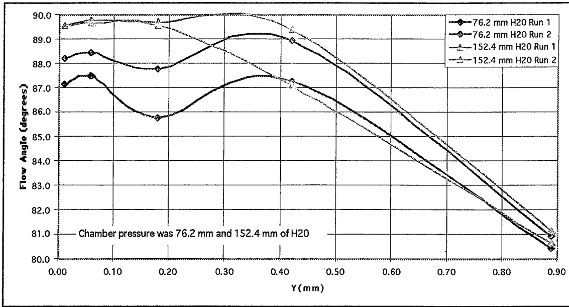
Figure G3. A radial survey through the pressurized window at a Prandtl of 0.9054
