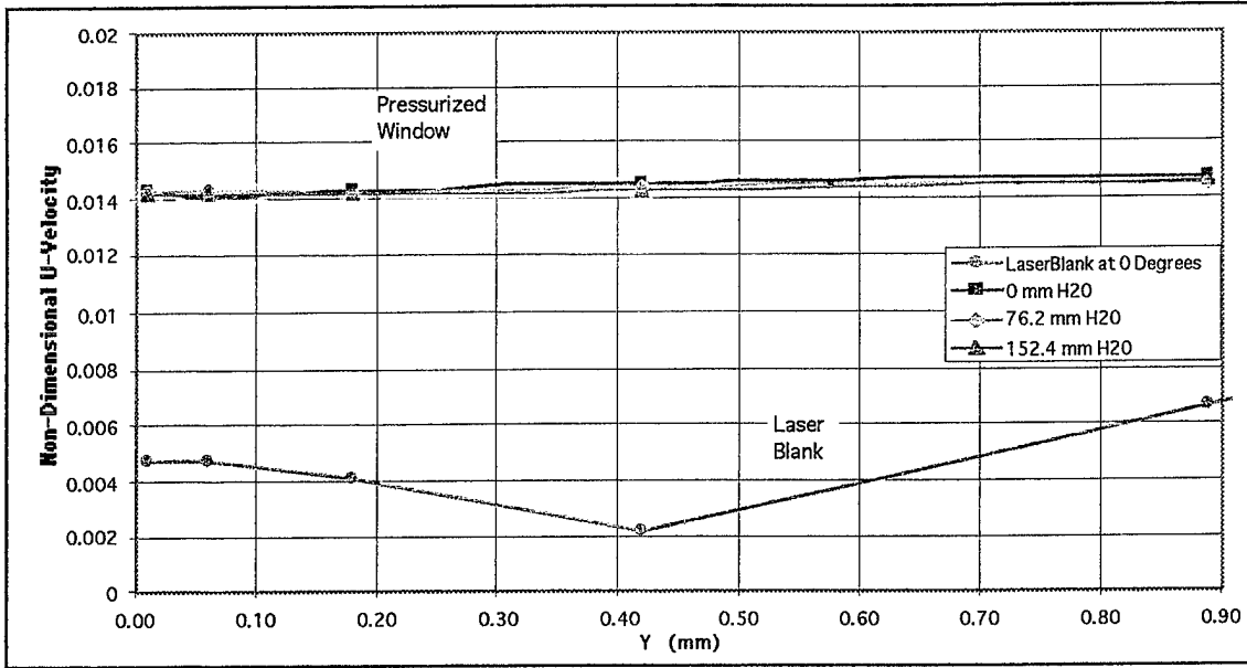
Figure 27a. Comparisons of radial surveys using the laser blank and pressurized LDV window at a Pr at of 0.9620
