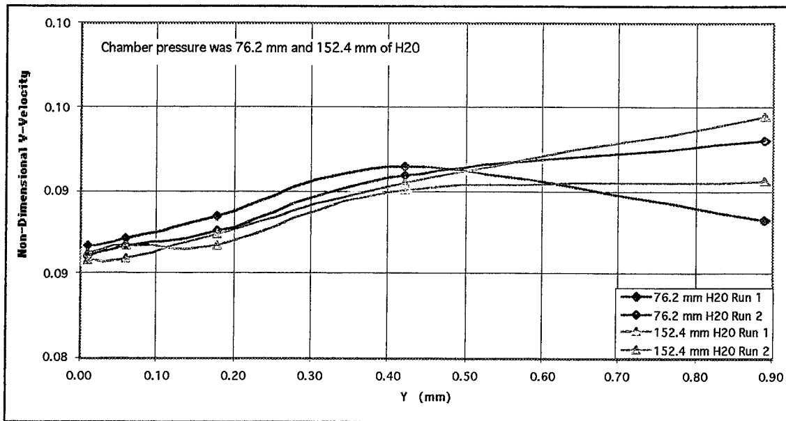
Figure G1b. A radial survey through the pressurized window at a Pr at of 0.9054
