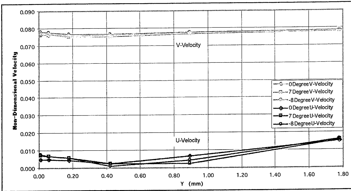
Figure 18. A radial survey through the laser blank at a Prandtl of 0.9620
