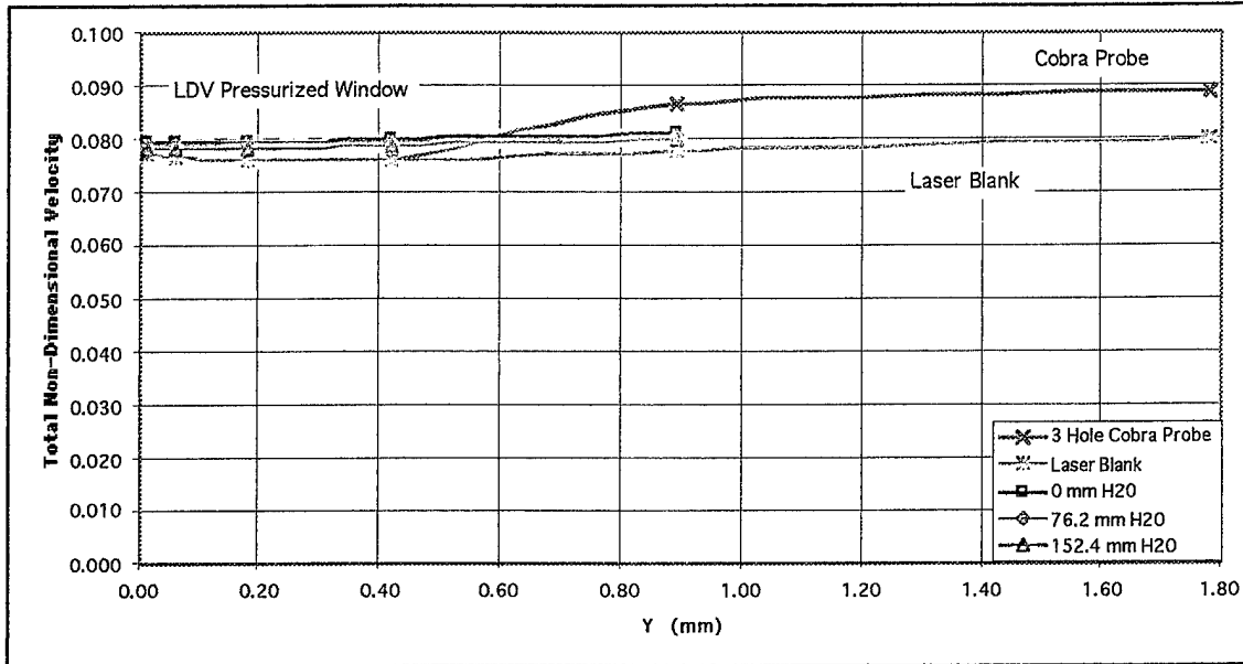
Figure 36. Final total non-dimensional velocity comparison between laser blank, pressurized window, and 3-hole cobra probe at a Prandtl of 0.9620
