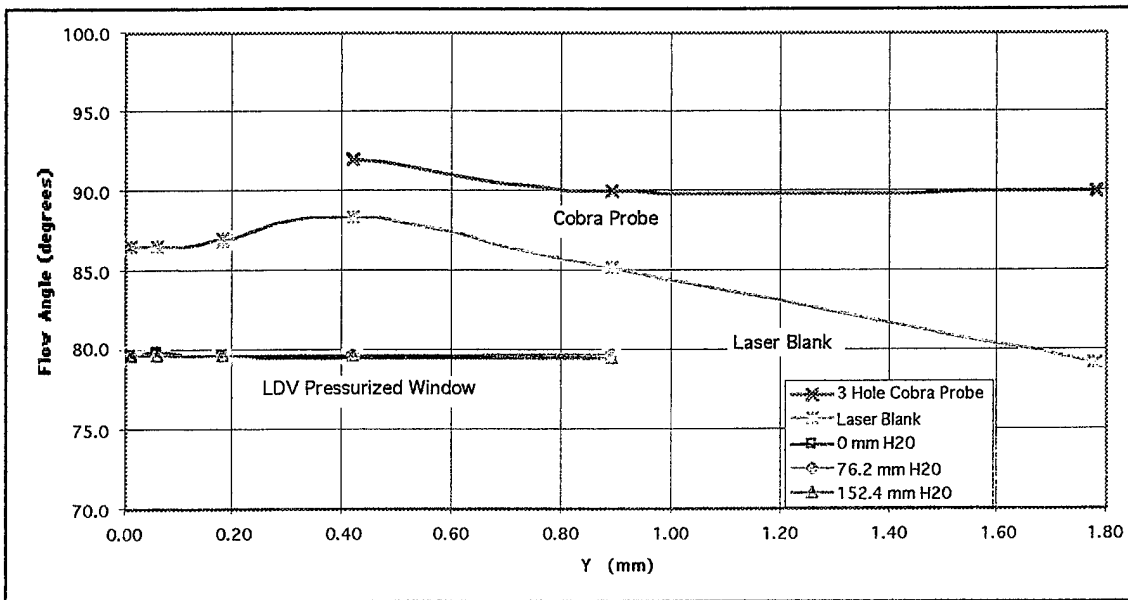
Figure 37. Final flow angle comparison between laser blank, pressurized window, and 3-hole cobra probe at a Prandtl of 0.9620
