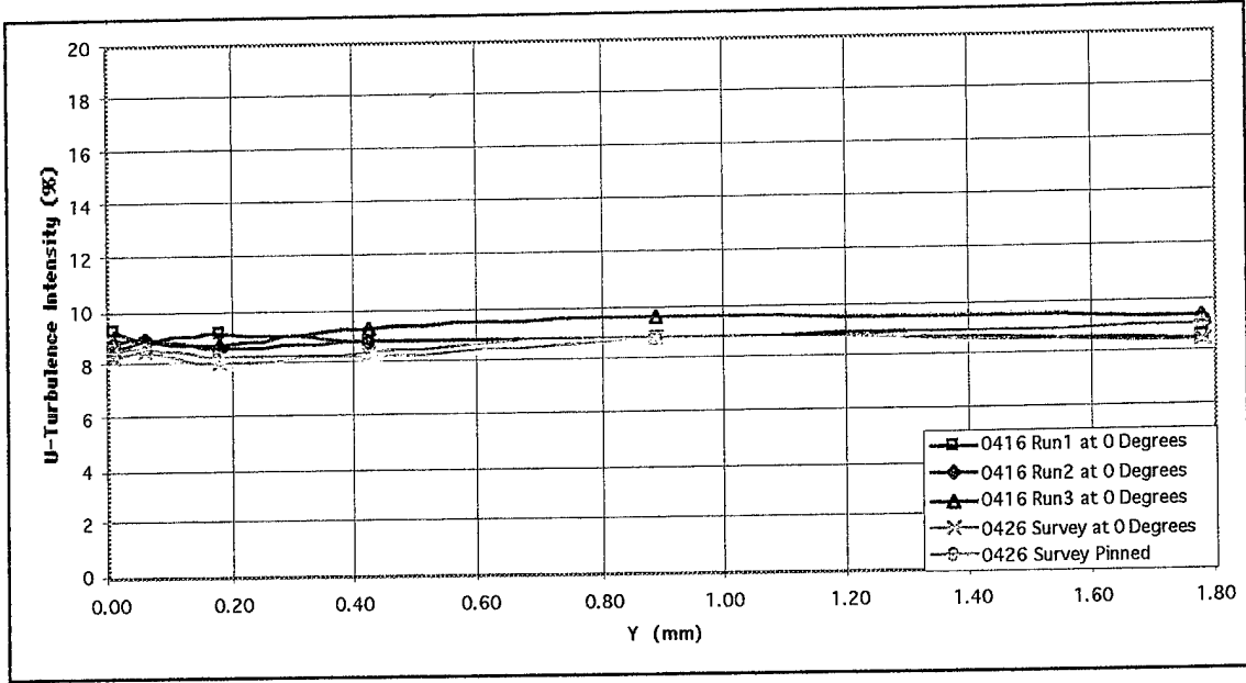
Figure 16a. A radial survey through the laser blank at a Prandtl number of 0.9054
