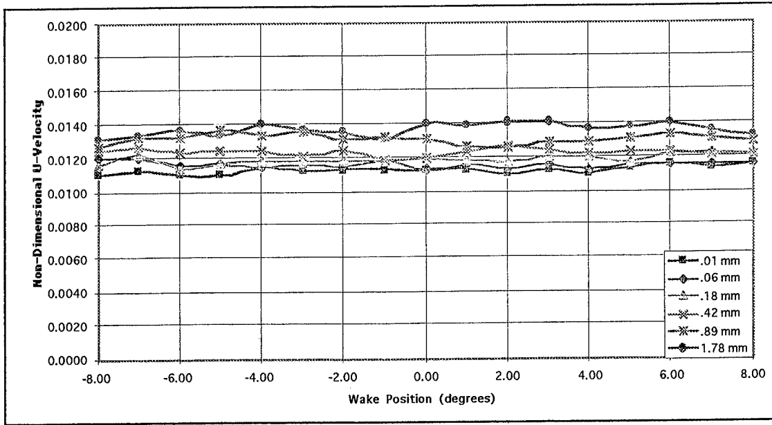
Figure 21a. A circumferential survey through the laser blank at a Prandtl of 0.9620
