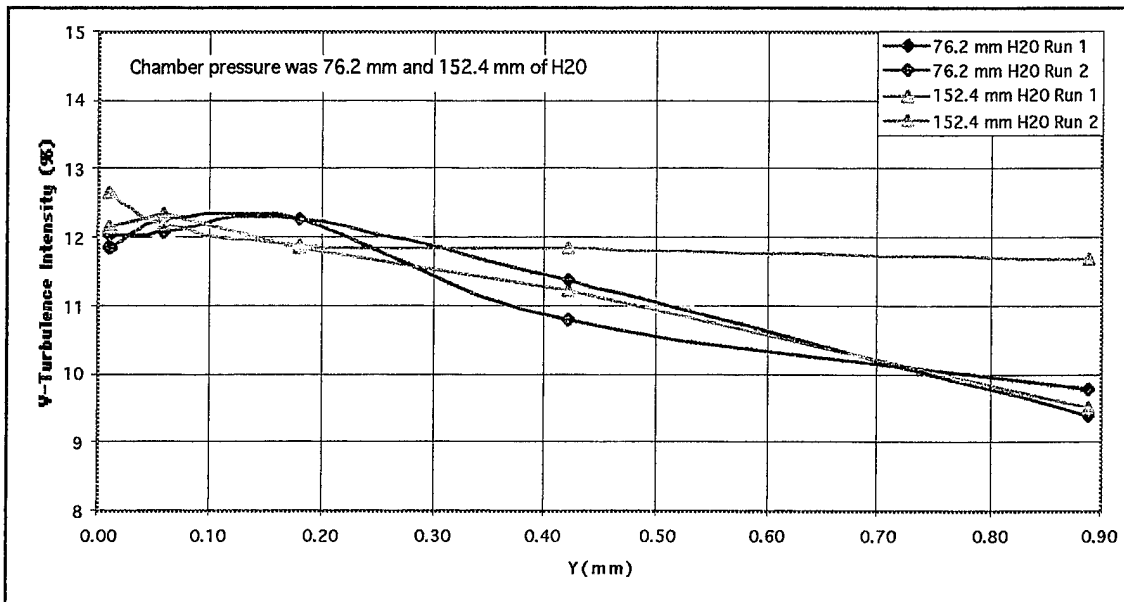
Figure G2b. A radial survey through the pressurized window at a Prandtl of 0.9054
