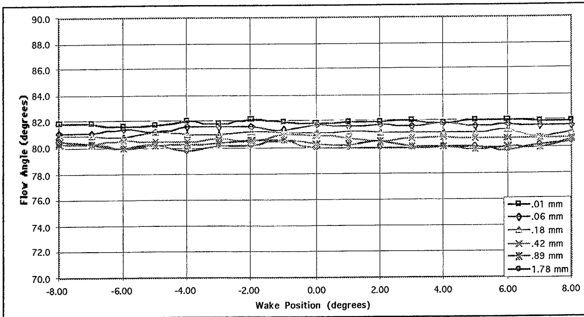
Figure 23. A circumferential survey through the laser blank at a Prandtl of 0.9620
