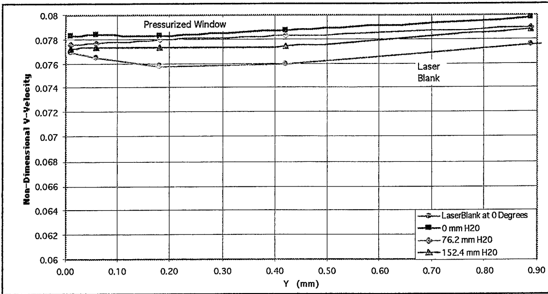
Figure 27b. Comparisons of radial surveys using the laser blank and pressurized LDV window at a Pr at of 0.9620
