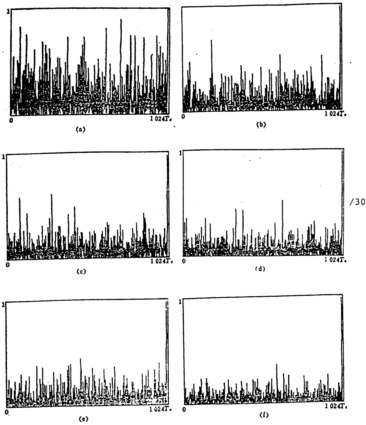
Fig.5 Sample Sequences Under Various Types of Signal to Noise Ratios A=2^{17} - 1 Gold Code Partial Sequence \overline{A} = -A (a) E_b/N_o = 4.0\text{dB} , (b) E_b/N_o = 5.0\text{dB} , (c) E_b/N_o = 6\text{dB} , (d) E_b/N_o = 7\text{dB} , (e) E_b/N_o = 7.5\text{dB} , (f) E_b/N_o = 8.0\text{dB} .
