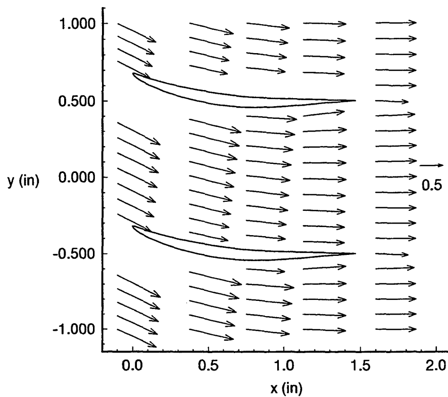
Figure 5.23. Streamwise Velocity Vectors for Moving Endwall t/c = 0.01 , z = 0.0 , Re_c = 9.72 \times 10^4
