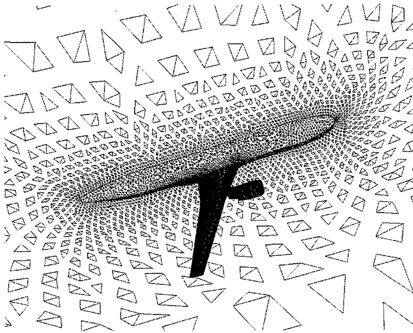
Figure 3: The same dataset, with only every fourth grid element displayed.
