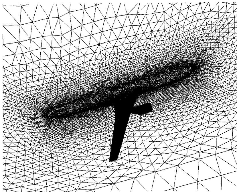
Figure 1: A surface mesh for the numerical simulation of airflow over a low-wing transport aircraft.
