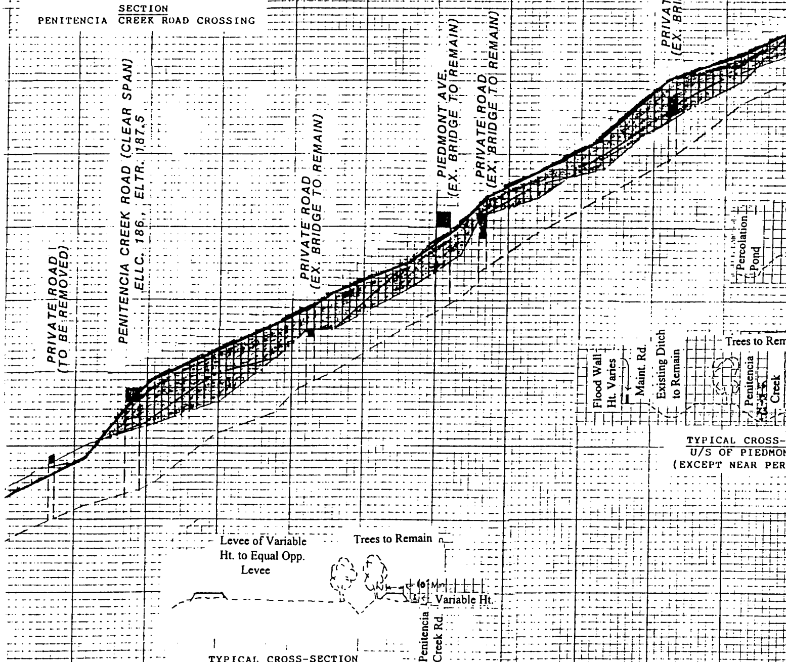
TYPICAL CROSS-SECTION UPPER PEN. RD. TO PIEDMONT AVE.
