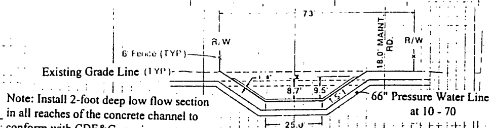
TYPICAL CROSS-SECTION D/S OF W.P.R.R.
