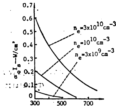
Fig. 5 Variation of maximum optical power density with electron density and gas temperature for \text{CO}_2\text{-N}_2\text{-He} (0.1-0.1-0.8) laser mixture at 10Torr
