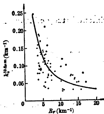
Fig. 3. Correlation between aerosol extinction coefficients at 10.6 μm and visibility
