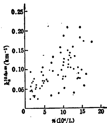
Fig. 2, Correlation between aerosol extinction coefficients at 10.6 μm and aerosol concentration
