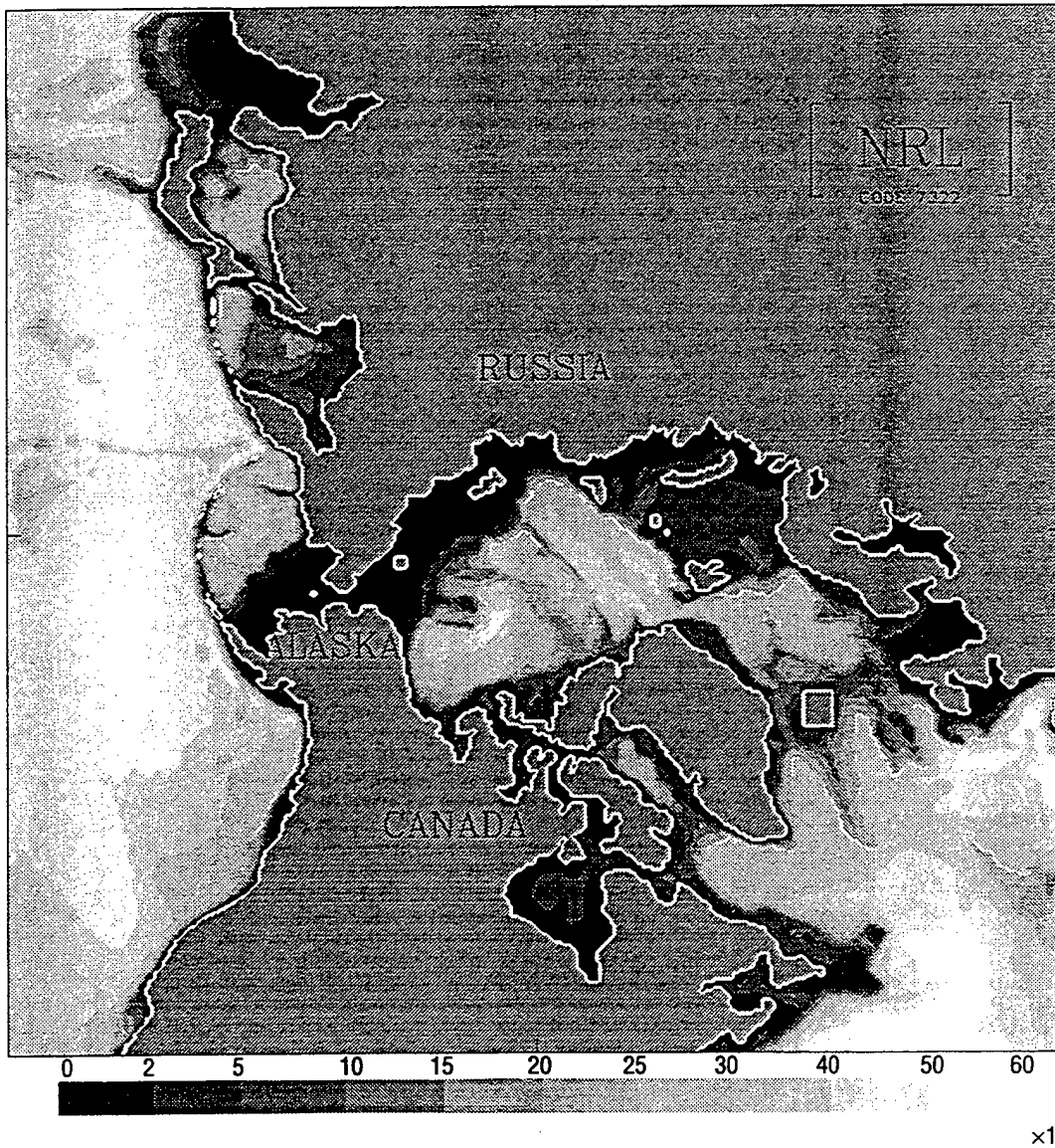
Fig. 9.1 — Bottom topography in PIPS2.0 domain according to ETOPO5. Scale range from 0–6000 m.
