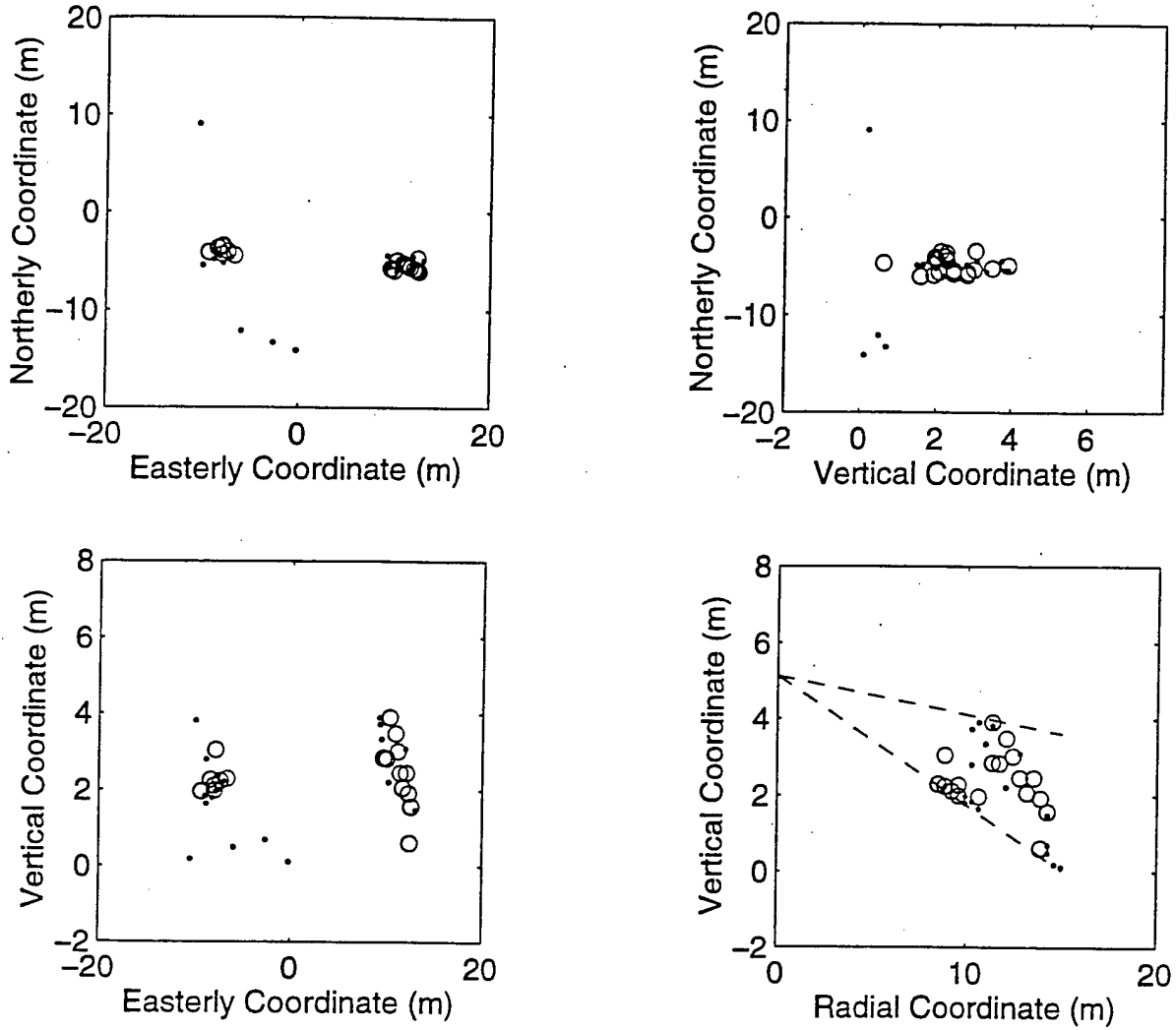
Target Locations, April, Scan 25, -40 < . < -35 < o
