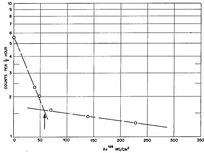
Figure 6. Al absorption of Compton recoils from the 0.42 Mev \gamma 's of Au 198 residual absorber was 94.7 mg/cm 2 end-point at 94.7 + 57.5 = 152.2 mg/cm 2 .
