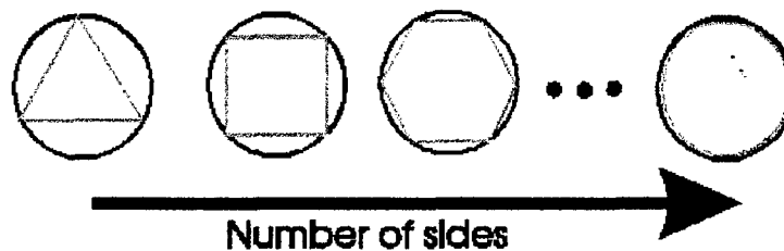
Figure 6-9: Geometric Shapes with Similar Properties
