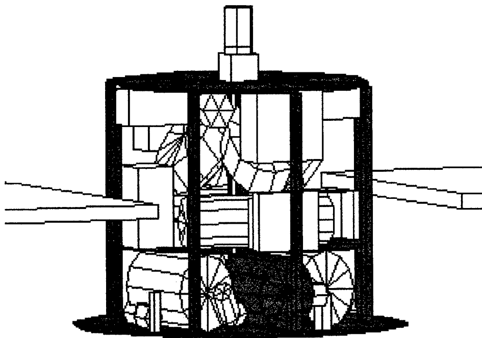
Figure 8-11: MAXTAC-N (deployed)
