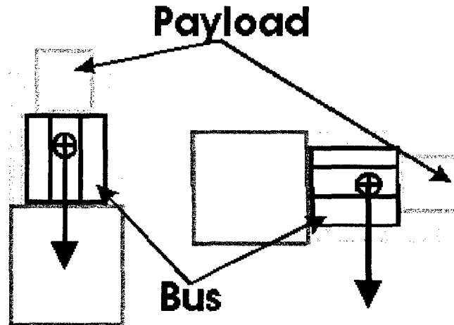
Figure 15-33: Axial and Lateral Loading on a Satellite Bus
