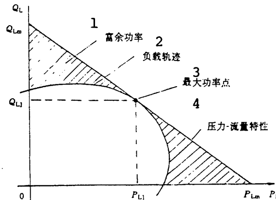
Fig. 11. Load track matched with load pressure-flux properties of valve KEY: 1 - surplus power 2 - load track 3 - maximum power point 4 - pressure-flux properties
