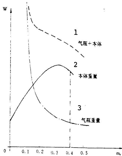
Fig. 9. Variation of body and air collector weight with m_r KEY: 1 - air collector + body 2 - body weight 3 - air collector weight
