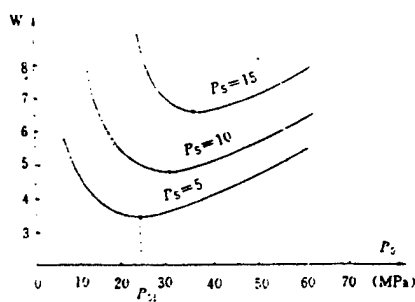
Fig. 5. Effect of control surface operating pressure P_s on air collector weight
