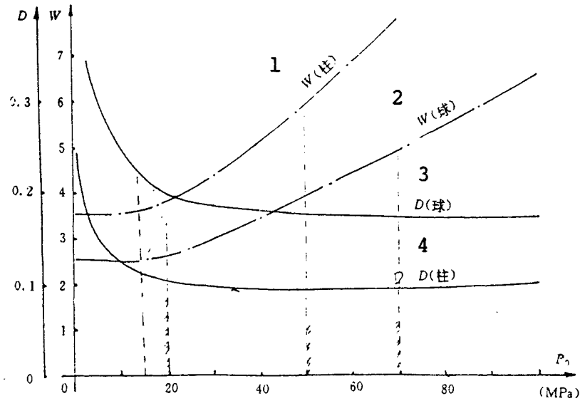
Fig. 4. Relationship between relative weight W and outer diameter D of air collector and gas storage pressure P_0 KEY: 1 - W (cylindrical) 2 - W (spherical) 3 - D (spherical) 4 - D (cylindrical)
