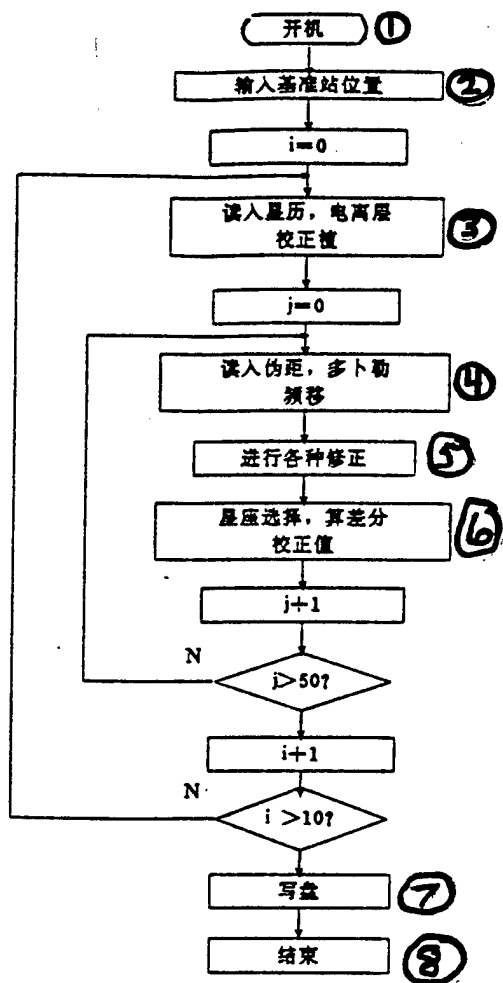
Fig.6 Long Range GPS Pseudorange Differential Datum Station Program Flow Chart
