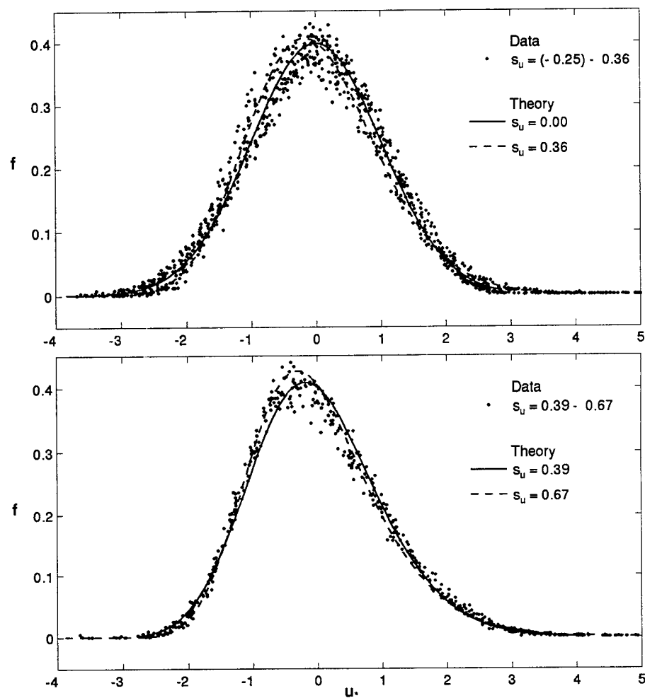
Figure 5.4: Measured and Computed Probability Distributions of Horizontal Velocities for Tests 1-3
