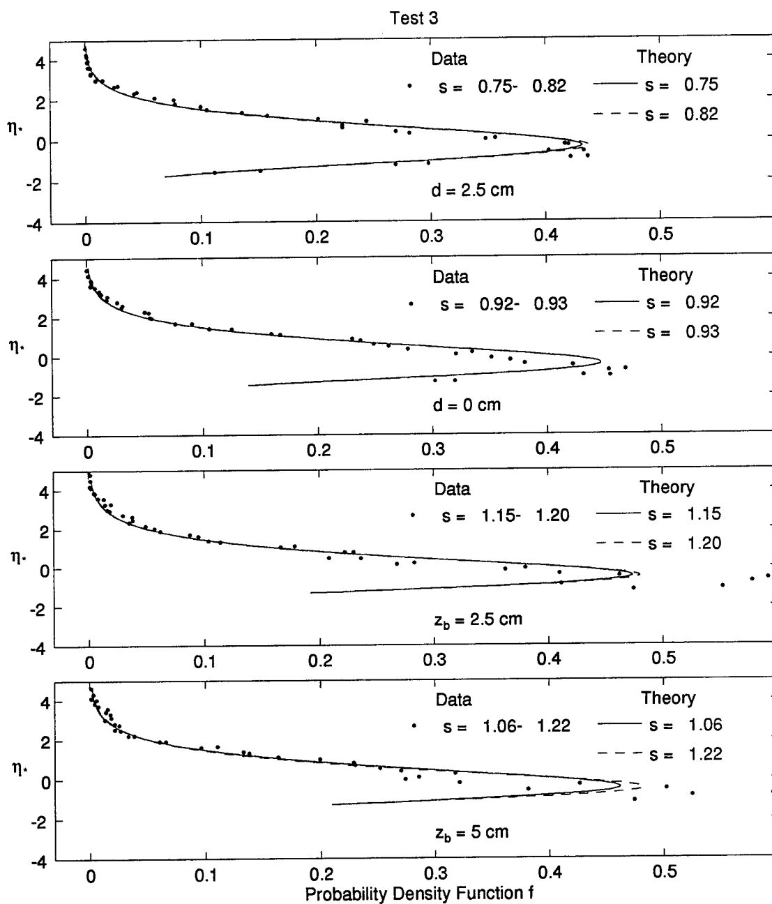
Figure 4.54: Measured and Computed Probability Distributions at Water Depth d = 2.5 and 0 cm and Bottom Elevation z_b = 2.5 and 5 cm for Test 3
