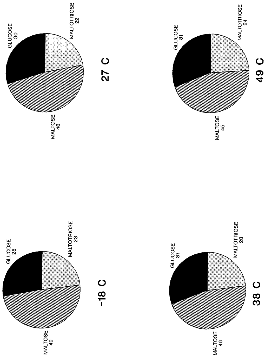
Figure 10. Composition of amylose digested carbohydrates in PBRD stored for 1 month at -18° to 49° C. Pretreatment: samples ground.
