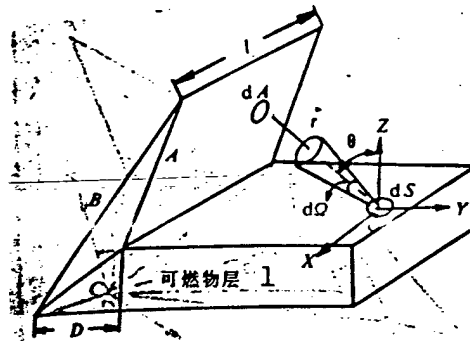
Fig. 1. Radiation model of flame zone in fire line KEY: 1 - combustible layer
