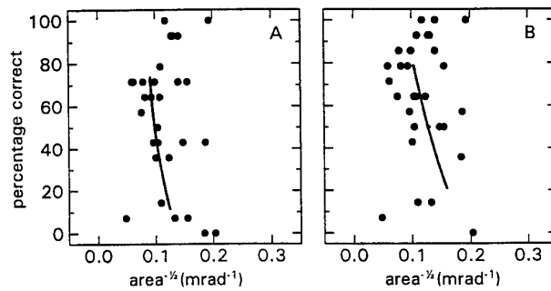
Fig. A27 Entire set of observer scores for Tankers as a function of (target area) -1/2 . See also Fig. A23.
