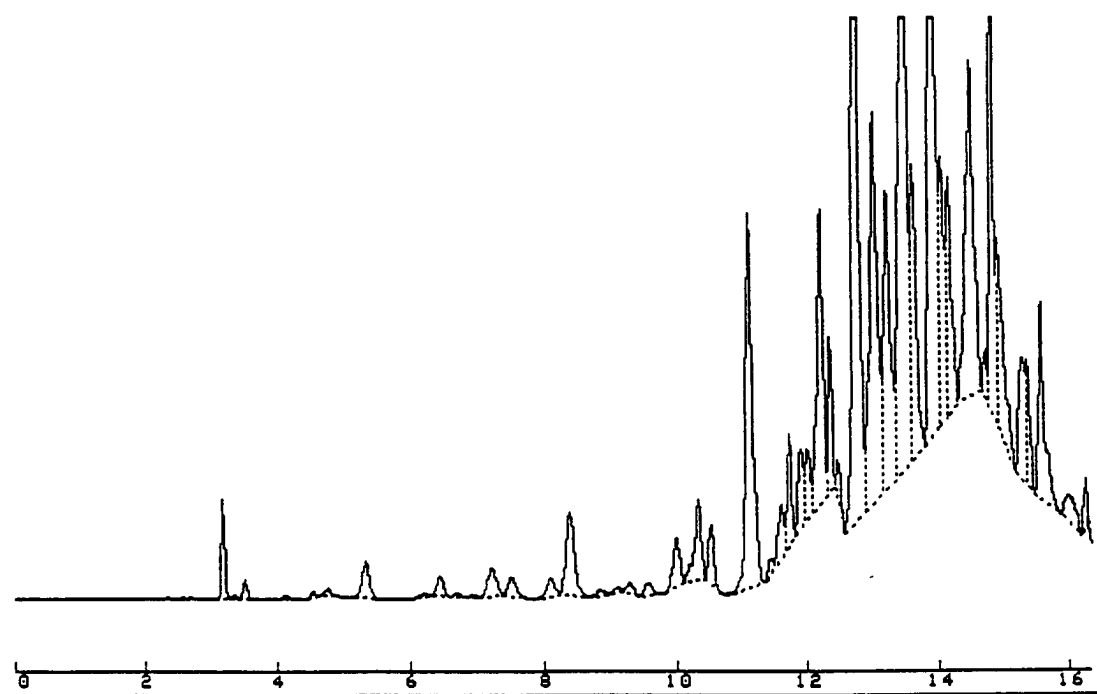
Figure 4. Example JP-4 (Total Volatiles) Standard Chromatogram
