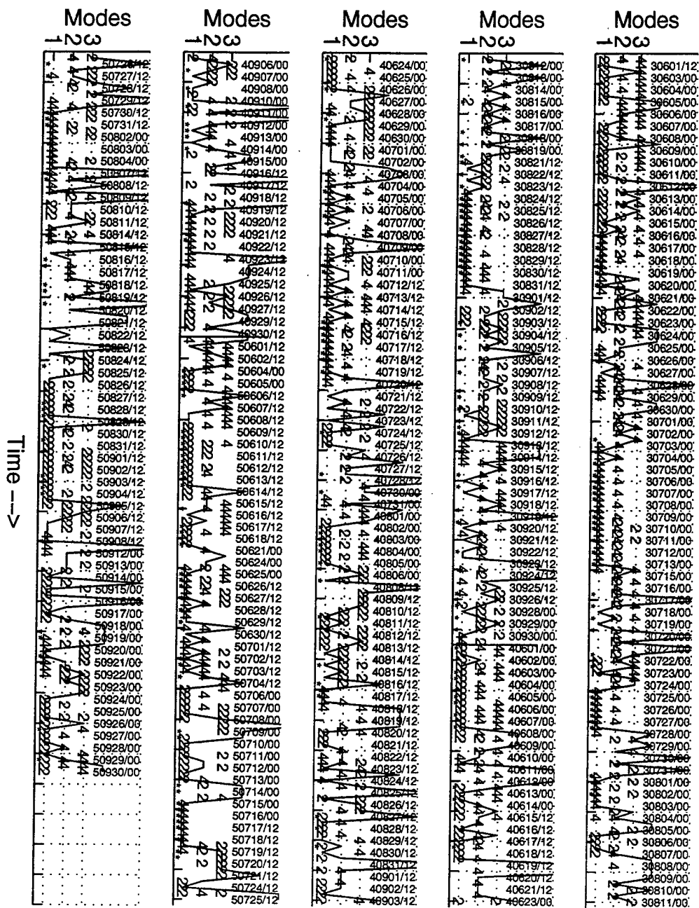
Figure 52. Plot of the distributions of the primary phases of VEOF modes 1-3 for every 12 hours. Plots of 2 and 4 in each mode represents principal components in the primary phases, while blanks represent components in the minor 1 and 3 phases. The solid line connects the magnitudes of the largest VEOF mode for each time period.
